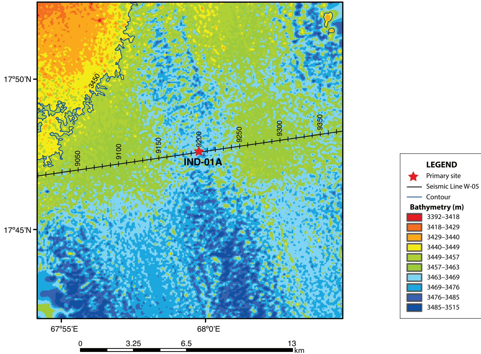
Figure AF1. Contoured bathymetric map showing seismic reflection profile Line W-05 (Fig. AF2) and the location of proposed primary Site IND-01A.
