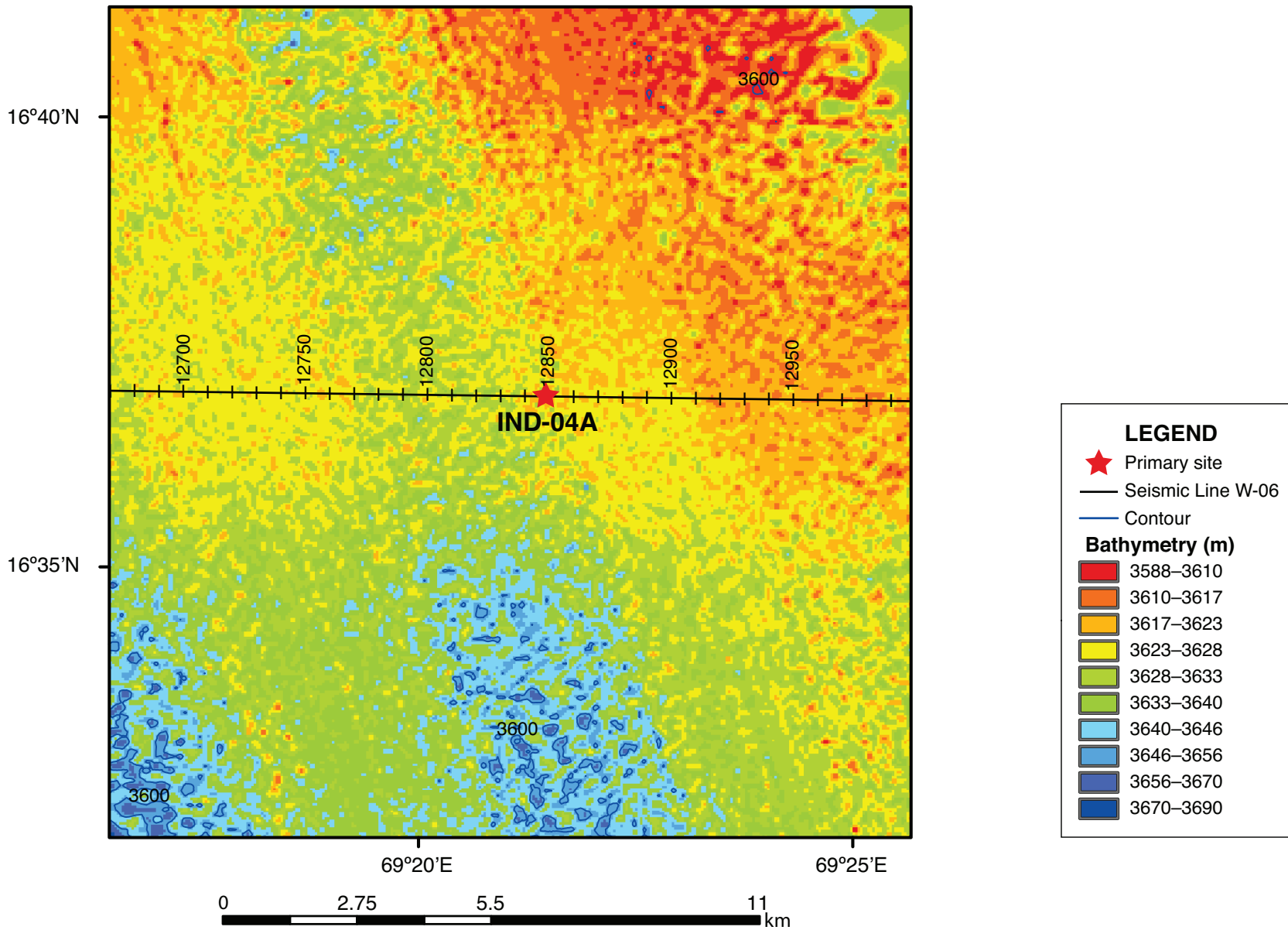
Figure AF7. Contoured bathymetric map showing seismic reflection profile Line W-06 (Fig. AF8) and the location of proposed primary Site IND-04A.
