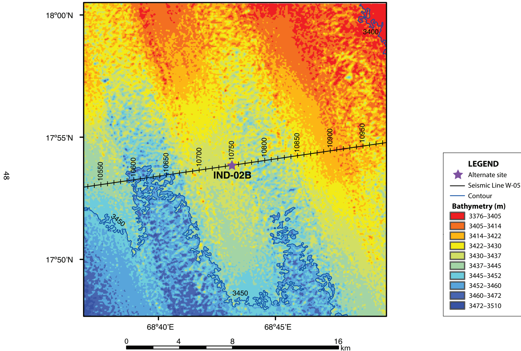
Figure AF3. Contoured bathymetric map showing seismic reflection profile Line W-05 (Fig. AF4) and the location of proposed alternate Site IND-02B.
