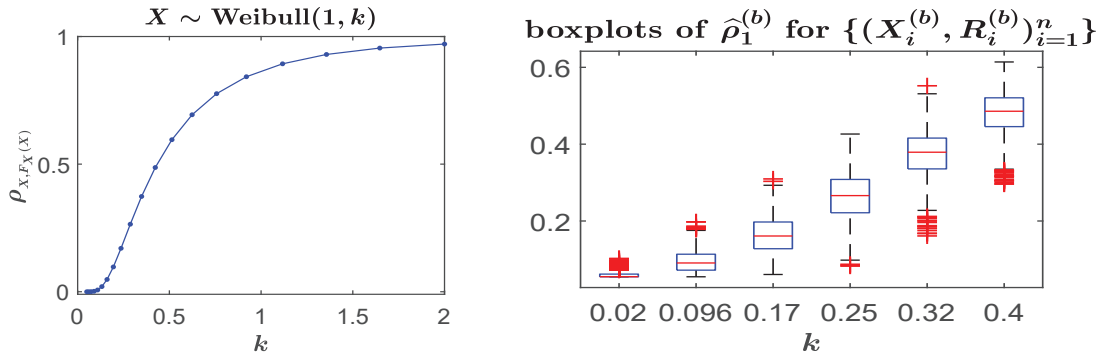
Figure 2: ( X \sim \text{Weibull}(1, k) ) Left panel: Plot of (21) versus k > 0 . Right panel: Boxplots of \hat{\rho}_1^{(b)} for \{(X_i^{(b)}, R_i^{(b)})\}_{i=1}^n , b = 1, \dots, N , with N = 1000 and n = 1000 , for X \sim \text{Weibull}(1, k) , with choices of k indicated below the boxplot.
