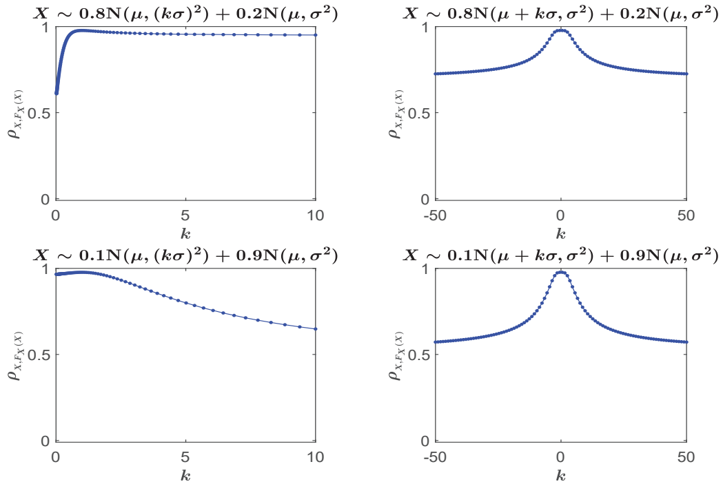
Figure 3: ( X \sim \text{mixture Gaussian distribution} ) Left panels: plot of \rho_{X, F_X(X)} versus k , where X \sim p\mathcal{N}(\mu, (k\sigma)^2) + (1-p)\mathcal{N}(\mu, \sigma^2) with p = 0.8 and p = 0.1 . Right panels: plot of \rho_{X, F_X(X)} versus k , where X \sim p\mathcal{N}(\mu + k\sigma, \sigma^2) + (1-p)\mathcal{N}(\mu, \sigma^2) with p = 0.8 and p = 0.1 .
