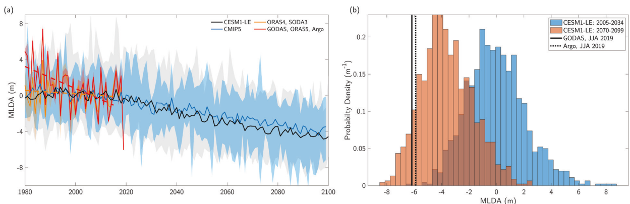
Fig. 2. (a) JJA MLDAs averaged in NEPac (black box, Fig. 1a) for two observational groupings (red/orange) and ensemble means of CESM1-LE (black) and CMIP5 (blue). Shading for each time series represents the full range (min-to-max) across respective ensembles. (b) Probability distributions of JJA ensemble mean CESM1-LE MLDAs averaged in NEPac during the “present” (blue; 2005–34) and “future” (orange; 2070–99). Vertical black lines mark JJA 2019 MLDA values from GODAS (solid) and Argo (dashed) data averaged in same region.
