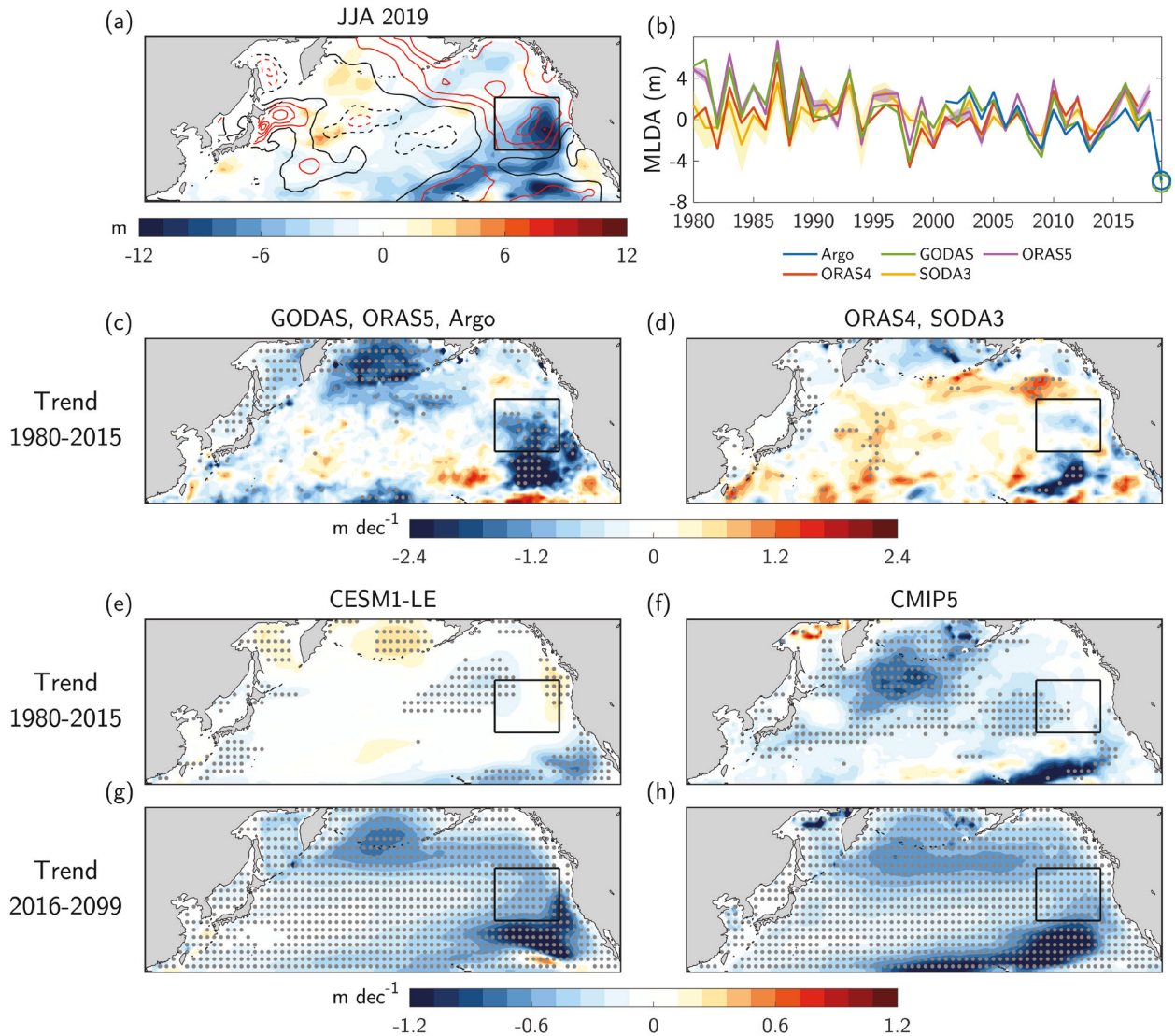
Fig. 1. (a) JJA 2019 MLDAs (m; shading) and SSTAs (°C; contours, positive solid and negative dashed) from Argo and GODAS, respectively. Contour interval is 0.5°C starting at 0.5°C (solid black). (b) MLDAs for five observational analyses (Table 1) averaged in the black box (i.e., 34°–47°N, 213°–232°W) shown in each map. Circles mark 2019 values. Shading for SODA3 and ORAS5 represents the full range (min-to-max) across respective ensembles. (c), (d) Observed JJA MLD trends (m decade -1 ; shading) from 1980 to 2015 averaged across two groupings: (c) GODAS, ORAS5, and Argo and (d) ORAS4 and SODA3. (e), (f) Simulated JJA MLD trend (m decade -1 ; shading) from 1980 to 2015 in ensemble means of CESM1-LE and CMIP5. (g), (h) As in (e), (f), but for the period 2016–99. All trends based on linear least squares fit. Stippling represents 95% significance for a Mann-Kendall test.
