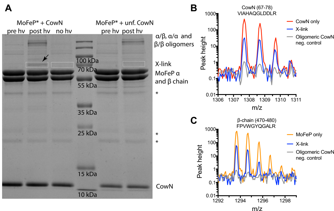
Figure 7. Cross-linking of MoFeP and CowN. A, SDS-PAGE of the cross-linking products between MoFeP* and CowN. The 70 kDa putative CowN-MoFeP cross-linked pair is marked with an arrow. The boxes represent the approximate regions of the gel that were excised for tryptic digest and MALDI-TOF MS analysis. Pre hv refers to samples at the start of the cross-linking reaction, post hv refers to samples that were illuminated for 30 min, whereas no hv represents identical samples that were incubated for 30 min without light. Bands marked by an asterisk represent impurities in MoFeP. The full gel in panel A can be found in the Supporting information . B, comparison of the 1307.69 m/z peak from the MoFeP*-CowN cross-linking sample, a CowN-only sample, and the MoFeP*-unfolded CowN negative control. C, same as in B, but for the 1293.67 m/z peak characteristic of MoFeP \beta -chain.
