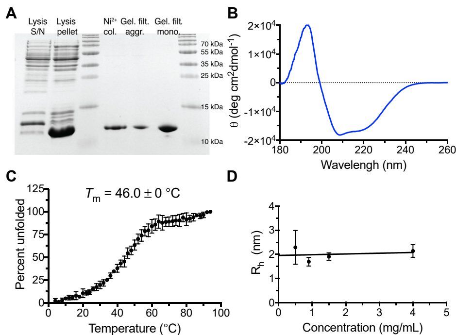
Figure 3. Purification and physical properties of CowN. A, SDS-PAGE of His-CowN in different stages of purification. B, CD spectrum of CowN showing predominantly \alpha -helical secondary structure. C, thermal denaturation curve of CowN. D, determination of CowN radius by DLS, where the y-axis intercept represents the concentration independent radius.
