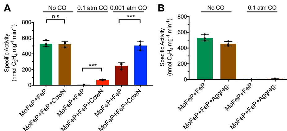
Figure 4. Effect of CowN on nitrogenase activity. A, nitrogenase C_2H_2 reduction in the presence and absence of CowN with no CO, 0.1 atm CO, or 0.001 atm CO. B, control experiments determining that unfolded CowN does not protect nitrogenase. MoFeP and FeP concentrations are 0.2 \mu M and 2 \mu M, respectively. In A and B, the CowN concentration is 2 \mu M. Activity differences that are significant to p = 0.001 are denoted by ***. n.s. means no statistical difference.
