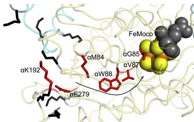
Figure 9. Possible CowN-binding site near a proposed hydrophobic CO access channel in Gd-MoFeP (PDB: 5KOH). Key residues that line the entrance and interior of the channel are highlighted in red and annotated using G. diazotrophicus nitrogenase numbering. The arrow represents the proposed CO migration route. Lys residues that surround the channel entrance and may mediate interaction with CowN are highlighted in black. The MoFeP \alpha -chain is colored in light yellow and the \beta -chain is colored cyan.
