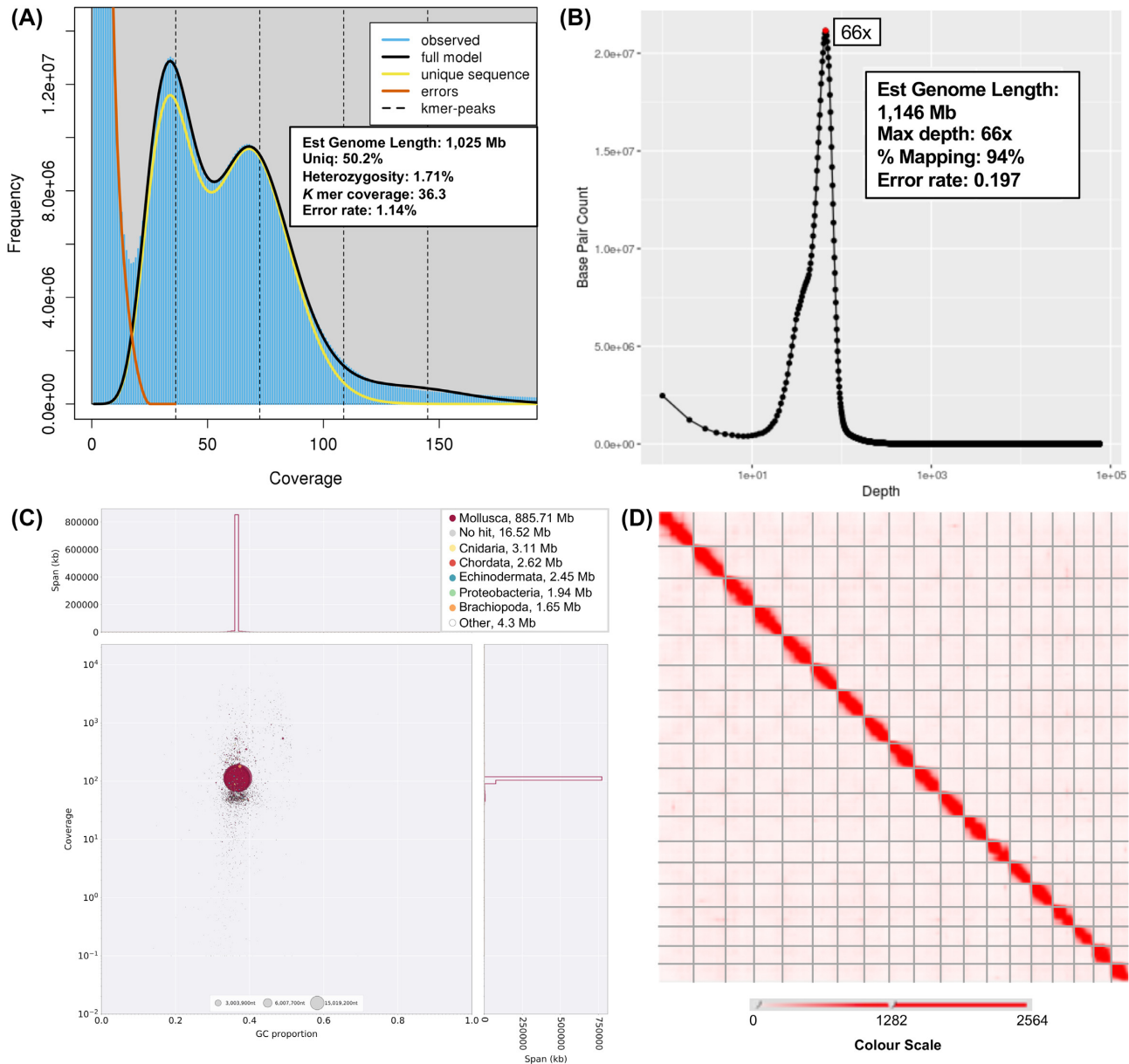
Figure 2: A, Genomescope2 [49] plot of the 21-mer k-mer content within the Pecten maximus genome. Models fitted and resulting estimates of genome size and read data as shown in figure. B, Base pair count by depth in PacBio data, determined using PBreads/Minimap2. C, Blobplot [50] of content of the P. maximus genome. Note that little-to-no contamination of the assembly can be observed, with the small amount of sequence annotated as non-metazoan mirroring the metazoan content in GC content and average coverage. Additional Blobplot plots and data, including those separated by phylum/superkingdom, can be found in Supplementary File 2. D, Hi-C contact map based on assembly created using 3D-DNA and Juicebox Assembly Tools (see [51] for an interactive version of this panel).
