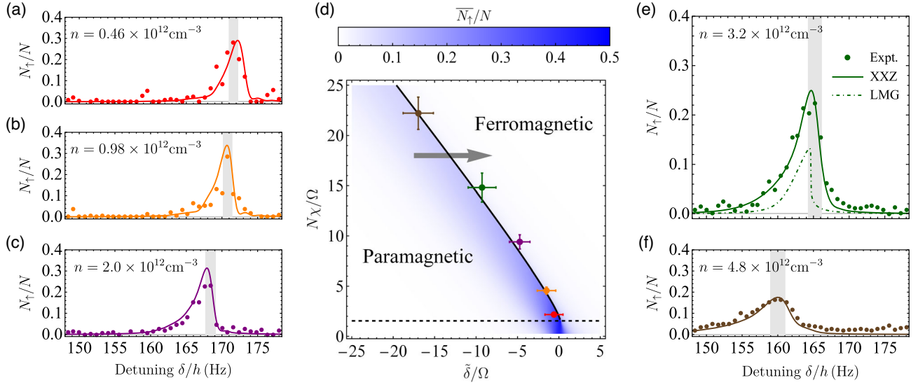
FIG. 3. (a)–(c), (e), (f) Dynamical phase transition in the 171 Hz blue sideband with mean atom density n = \{0.46, 0.98, 2.0, 3.2, 4.8\} \times 10^{12} \text{ cm}^{-3} , indicated by the asymmetric line shape after evolution time 0.5 s. The shaded areas indicate the critical points, where the uncertainty is set by finite frequency step of detuning as well as fluctuations in atom density and Rabi frequency. The filled circles denote experimental data, the solid lines denote mean-field theoretical predictions by H_{XXZ} , and the green dot-dashed line in (e) denotes the order parameter \overline{N_{\uparrow}}/N predicted by H_{\text{LMG}} (see text). We do not directly add the experimental error bars to the line shape data in (a)–(c), (e), (f) for visual reasons, and the typical statistical uncertainty in each figure is \Delta N_{\uparrow}/N = \{0.038, 0.020, 0.013, 0.010, 0.011\} , respectively. (d) Phase diagram for ferromagnetic to paramagnetic dynamical phase transition. The black solid line denotes the sharp phase boundary of DPT, the black dashed line separates the smooth crossover regime (below) with DPT regime (above), and the gray arrow illustrates the probing direction on phase diagram. The phase boundary is reconstructed from the critical points in (a)–(c), (e), (f) using the same choice of color to label data points.
