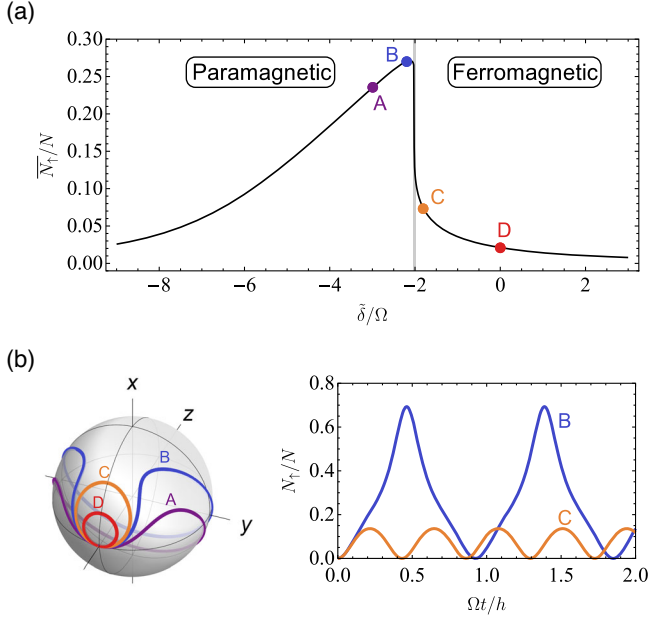
FIG. 2. (a) Dynamical phase transition (DPT) in LMG model with N\chi/\Omega = 5 , indicated by the sharp behavior in longtime average excitation fraction \overline{N}_{\uparrow}/N . The critical point is marked by the vertical gray line at \tilde{\delta}/\Omega = -2.02 , separating the dynamical paramagnetic phase (left) and the dynamical ferromagnetic phase (right). (b) Mean-field dynamics of the LMG model with \tilde{\delta}/\Omega = -3 (A), -2.2 (B), -1.8 (C), 0 (D). The left panel shows the mean-field trajectories on the Bloch sphere, and the right panel presents the mean-field evolution of the excitation fraction for trajectory B and C. The sharp change in dynamics between trajectory B and C also signals the DPT.
