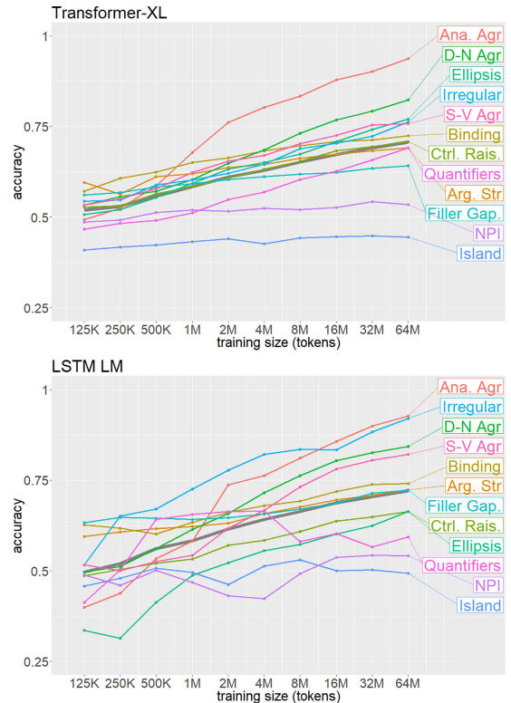
Figure 5: Transformer-XL (top) and LSTM LM (bottom) performance as a function of training size and phenomena in BLiMP. The gray line shows the average across all phenomena.
