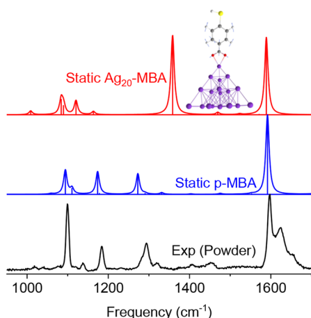
Figure 3. Experimental powder spectrum (black, 633\text{ nm} , 50\text{ }\mu\text{W}/\mu\text{m}^2 ) is shown along with the simulated spectra of the isolated (blue) and \text{Ag}_{20} -bound (red) MBA complex. The inset shows the structure of the \text{CO}_2 -Ag bound complex.
