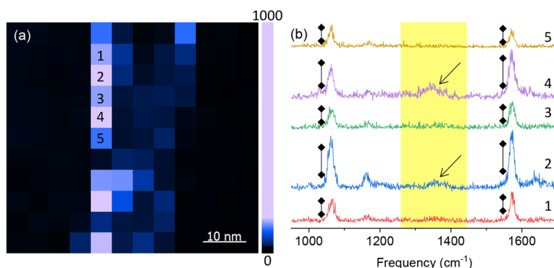
Figure 4. Zoomed in TERS image, tracing the edge of a silver nanocube (centered to the left of the image shown in panel a). Several pixels are enumerated in (a) and plotted in (b). They show the prevalence of the CO 2 -bound vs S-bound MBA. See text for more discussion.
