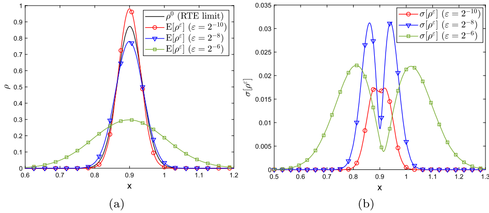
Fig. 10. (a) The plot compares particle density \mathbb{E}[\rho^\epsilon] for different \epsilon with \rho^0 , defined in (4.25) at t = 0.4 . (b) The plot shows the standard deviation of particle density \sigma[\rho^\epsilon] at t = 0.4 for different \epsilon . The random perturbation is of O(\epsilon) scale (4.31) with Gaussian \xi_{ij} in the two plots.
