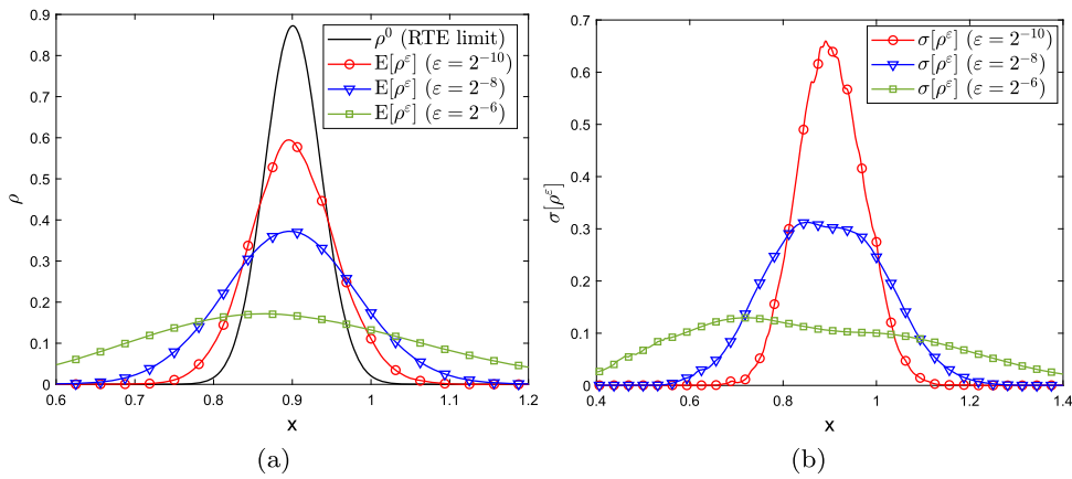
Fig. 11. (a) The plot compares particle density \mathbb{E}[\rho^\epsilon] for different \epsilon with \rho^0 , defined in (4.25) at t = 0.4 . (b) The plot shows the standard deviation of particle density \sigma[\rho^\epsilon] at t = 0.4 for different \epsilon . The random perturbation is of O(\epsilon^{0.4}) scale (4.32) with Gaussian \xi_{ij} in the two plots.
