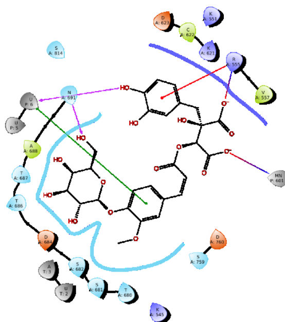
Figure 7. The interaction of SN00303170 with RdRp complex. Primer and template strands are colored red and cyan, respectively.
