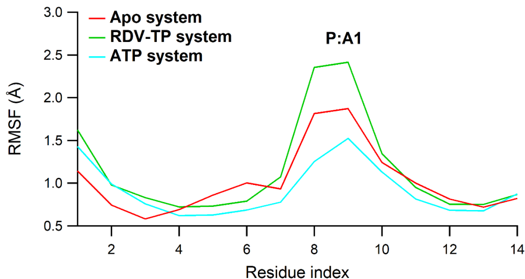
Figure 5. RMSF plot of RNA main atoms. Apo RdRp, RDV-TP, and ATP complexes are colored red, green, and cyan, respectively.
