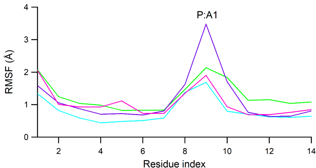
Figure 10. Plot of RNA residue fluctuation was recorded as RMSF values as RDV-TP (green) SN00166900 (cyan), SN00303170 (purple), and SN00359915 (pink).
