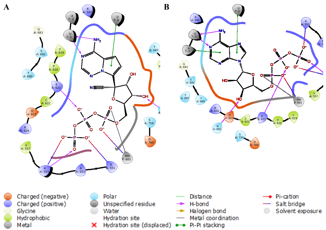
Figure 2. The detailed interaction of docked RDV-TP ( A ) and ATP ( B ) with RdRp.
