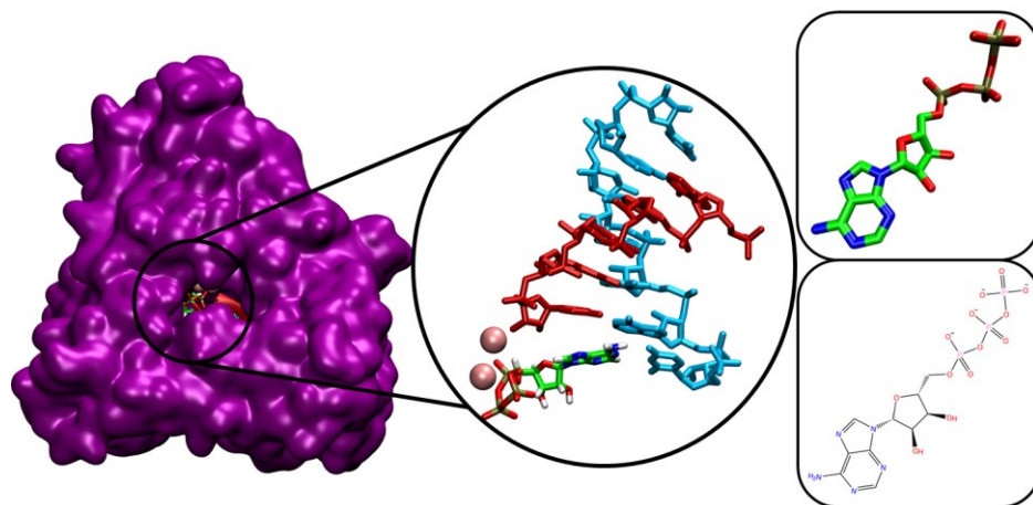
Figure 1. The 3D poses of RDV-TP (A) and ATP (B) in the RdRp SARS-CoV-2 model. Primer and template strands are colored red and cyan, respectively.
