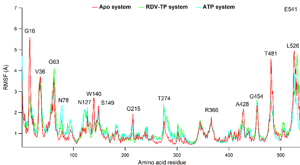
Figure 4. RMSF plot of protein. Apo RdRp, RDV-TP, and ATP complexes are colored red, green, and cyan, respectively.
