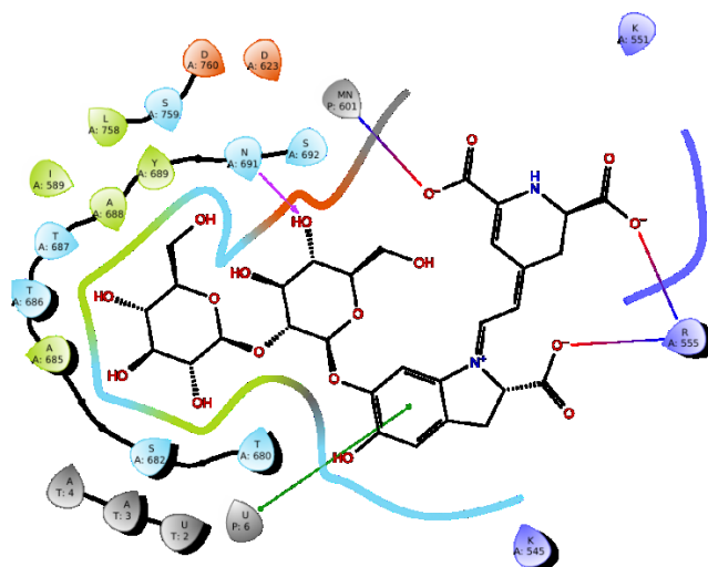
Figure 6. The interaction of SN00166900 with RdRp complex. Primer and template strands are colored red and cyan, respectively.
