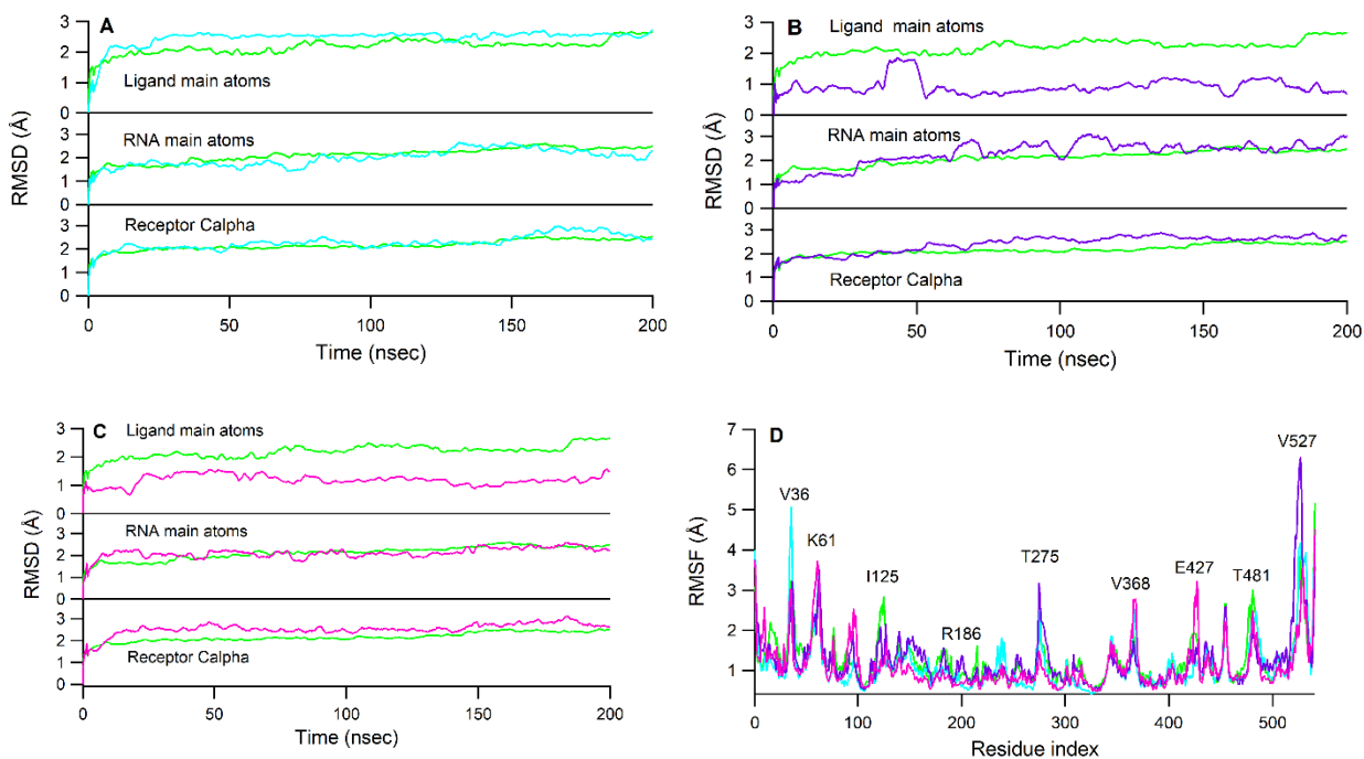
Figure 9. The RMSD values of RDV-TP and SN00166900 (A), RDV-TP and SN00303170 (B), RDV-TP and SN00359915 (C), and RMSF (D) values for each complex. RDV-TP, SN00166900, SN00303170, and SN00359915 are colored green, cyan, purple, and pink, respectively.
