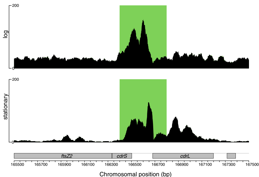
FIG 2 CdrL binds to the promoter region upstream of the cdrS-ftsZ2 operon. Raw sequencing data for immunoprecipitated samples are indicated by the black traces. Overlaid green boxes represent genomic regions detected by the MOSAiCS peak detection algorithm (see Materials and Methods) to be significantly enriched for binding of CdrL relative to the input control. The y-axis scale represents read counts. The CdrL binding site is shown for logarithmic-phase cells (top) and stationary-phase cells (bottom). Gray labeled boxes at the bottom represent genes (reverse strand).
