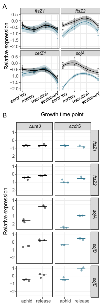
FIG 7 CdrS is important for wild-type expression levels of growth and cell division genes. (A) NanoString gene expression over the growth curve. Points represent log 10 -normalized expression data. Shaded regions represent smoothed conditional means. Labels on the x axis correspond to growth phases. (B) Expression data in response to cell division block with aphidicolin. Labels on x axis: aphid, gene expression during aphidicolin block; release, expression following washout. Points represent raw data; lines represent medians. Blue lines and points represent \Delta cdrS ; black, \Delta ura3 parent strain.
