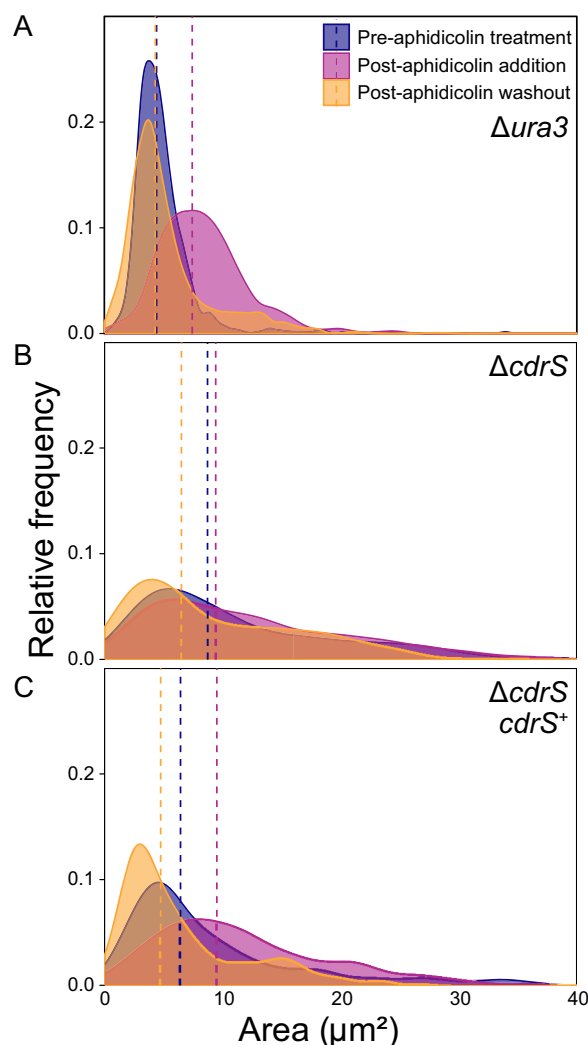
FIG 4 ΔcdrS is insensitive to cell cycle inhibitor aphidicolin. Cell area distributions are shown for the Δura3 parent strain (A), the ΔcdrS strain (B), and the complementation strain (C). Colors (as indicated in the legend): blue, before drug addition; pink, after 6 h of exposure to aphidicolin; orange, 11 h after removal of the drug by washing. Dotted lines indicate the geometric mean for each time point.
