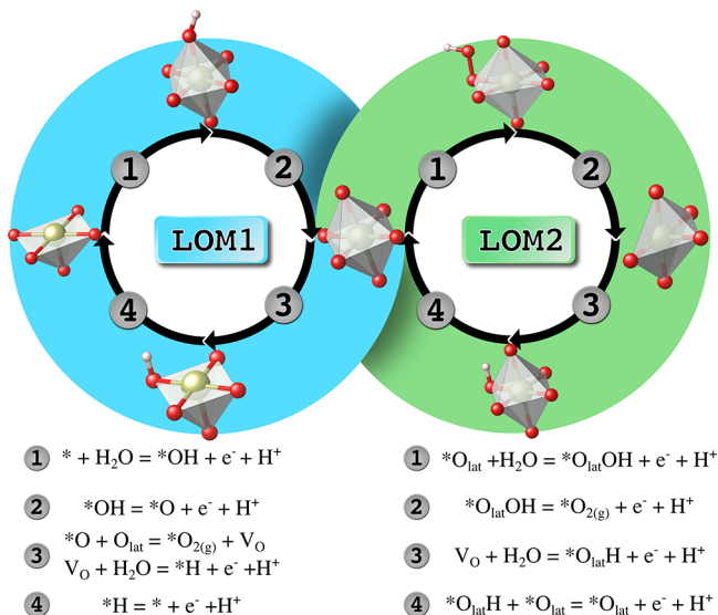
Scheme 1. Schematic Showing Two Major Mechanisms of the Lattice Oxygen Participation in the OER a
