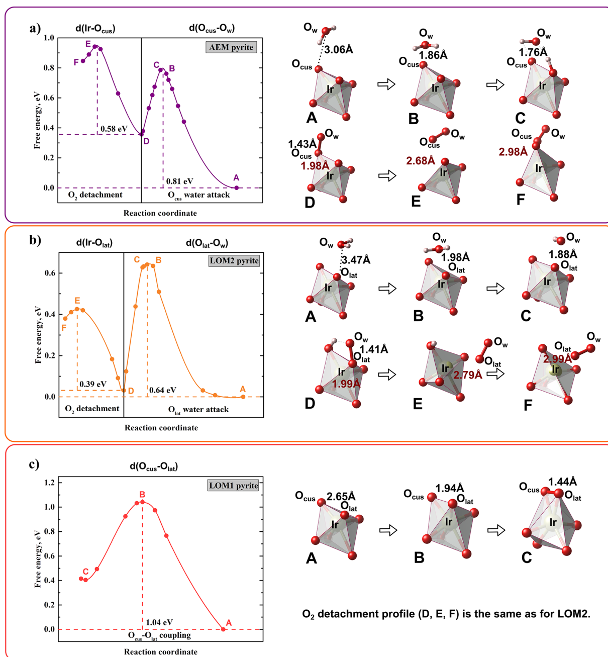
Figure 2. Free-energy profiles from AIMD thermodynamic integration simulations for \text{O}_2 formation and desorption steps along the AEM (a), LOM2 (b), and LOM1 (c) pathways over the pyrite (100) surface with three Ir vacancies (see the atomic structure in Figure S3). Atomic structures of the intermediate states with the distances along two collective variables are also presented. We note that for both AEM and LOM2 the first proton from attacking \text{H}_2\text{O} spontaneously adsorbs on the adjacent \text{O}_{\text{cus}} site, while the second proton is either transferred to solution for AEM or occupies the same \text{O}_{\text{cus}} site for LOM2.
