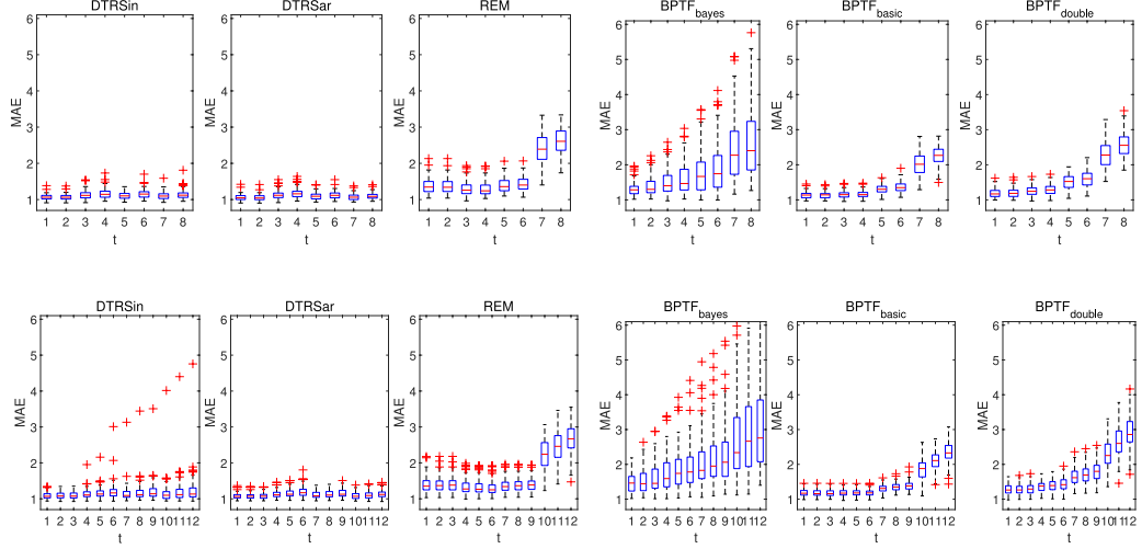
Figure 4: Box plots of the MAE for forecasting values with 8 and 12 time points and the true AR-1 correlation.
