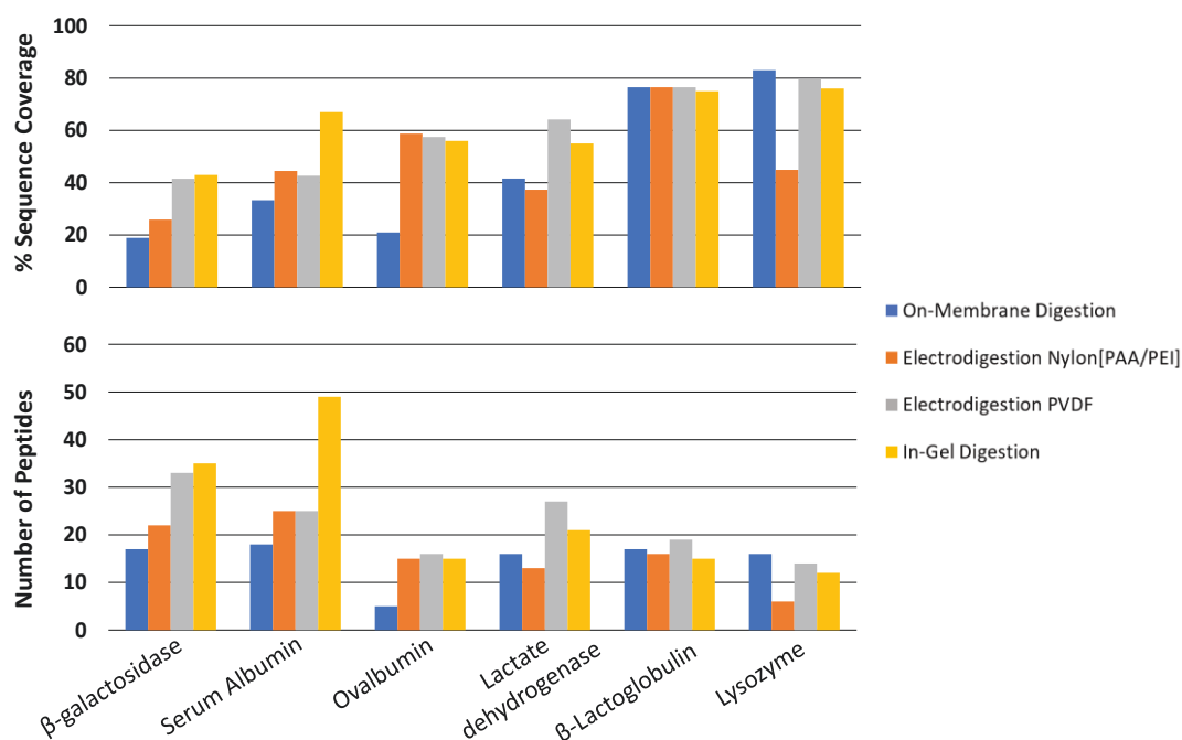
Fig. 2 Number of peptides and % sequence coverage in the analysis of a standard protein mixture using electrophoresis and the four different protocols in Fig. 1 . The number of peptides includes all peptides found from any piece of capture membrane or gel in either of the two replicates without redundancy.
