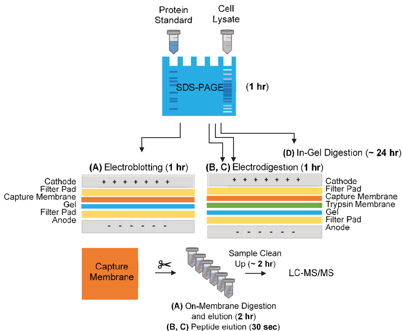
Fig. 1 Four methods for analysis of proteins separated using gel electrophoresis. (A) Electroblotting onto PVDF before on-membrane digestion and extraction. (B) Digestion during electroblotting, capture on polyelectrolyte-modified nylon, and peptide elution. (C) Digestion during electroblotting, capture on PVDF, and peptide elution. (D) In-gel digestion using a multistep procedure (not shown).
