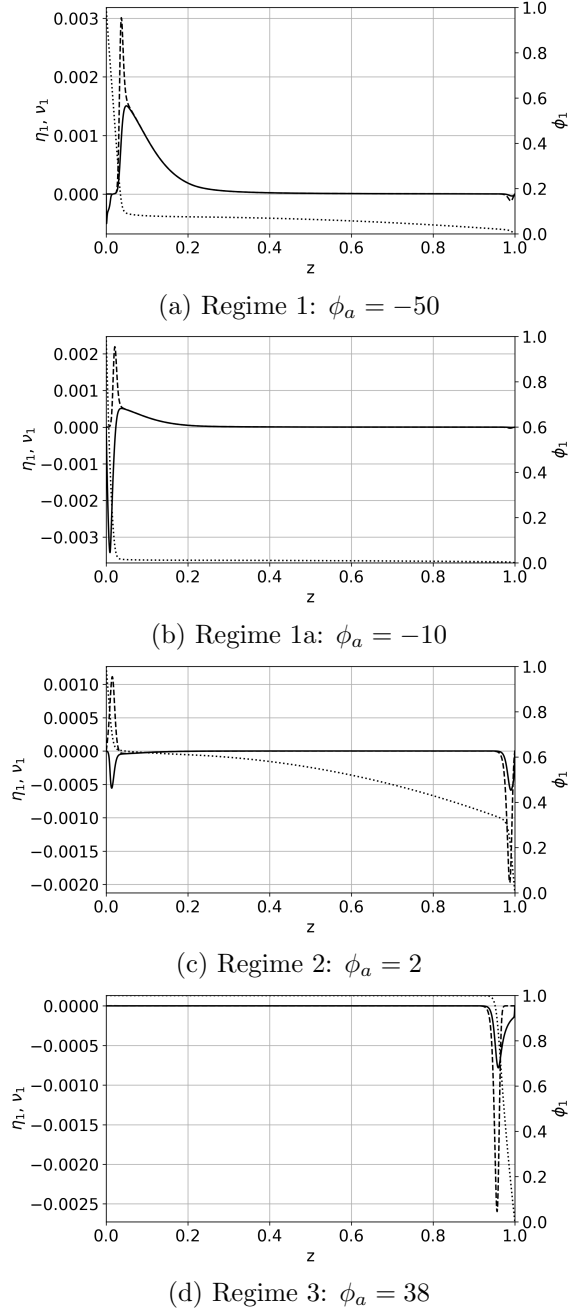
Figure 7: Sensitivity of the \eta (solid), \nu (dashed), and \phi (dotted) solutions per unit change in applied voltage, \phi_a . The conditions are in (a) regime 1, (b) regime 1a, (c) regime 2, (d) regime 3.
