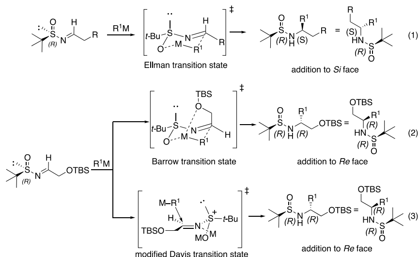
Figure 3. Transition-state hypothesis rationalizing the reversal of diastereoselectivity in the addition to \alpha -alkoxy imines.
