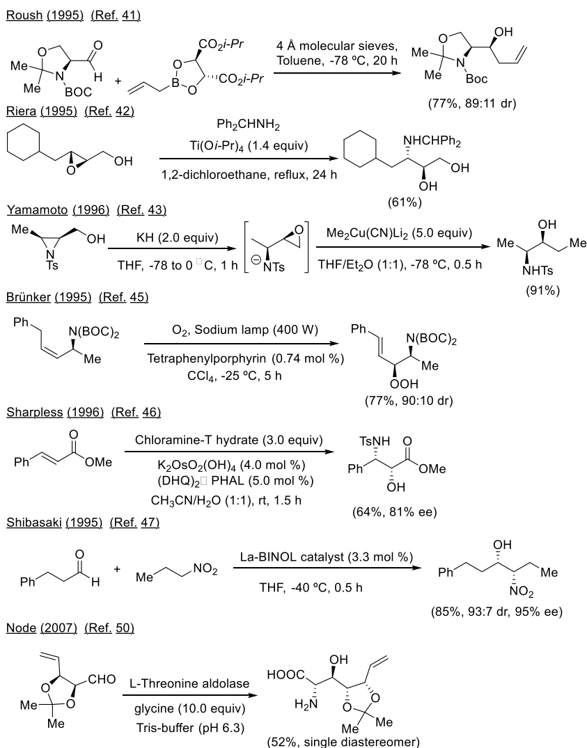
Scheme 3. Examples of Asymmetric Synthesis of 1,2-Amino Alcohols
