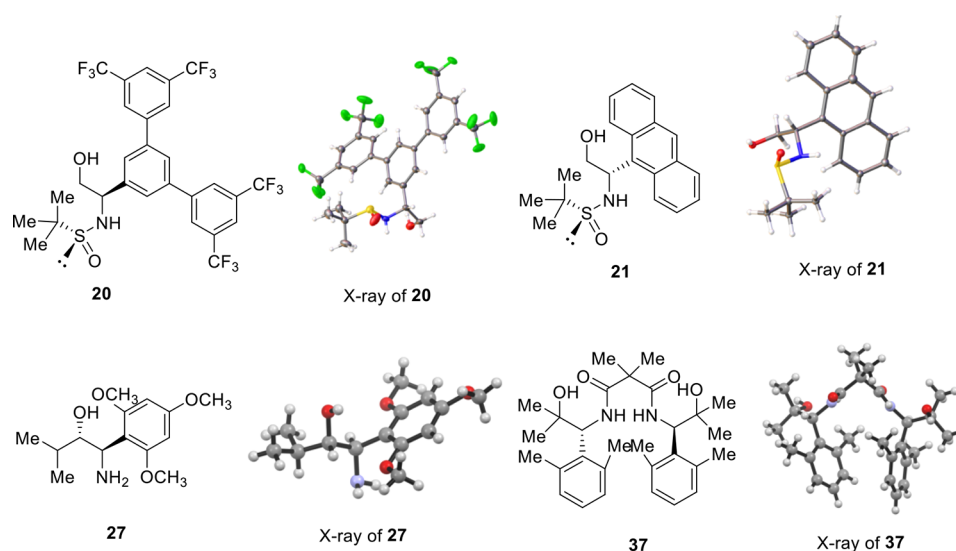
Figure 2. X-ray crystal structures of compounds 20, 21, 27, and 37.
