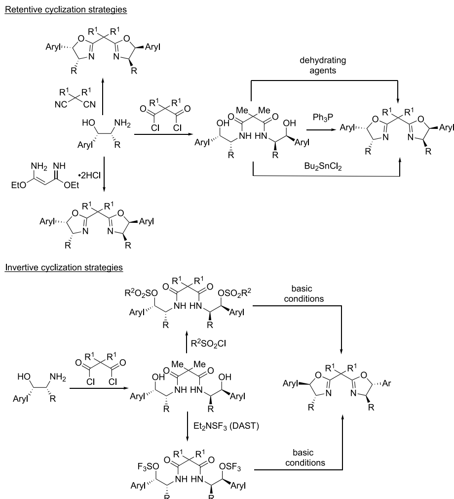
Scheme 4. Various Strategies for the Retentive and Invertive Construction of BOX Ligands
