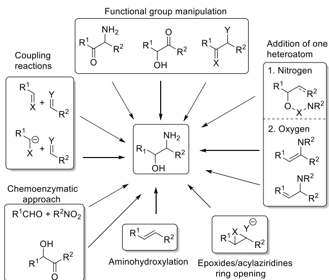
Scheme 2. Various Approaches for the Synthesis of 1,2-Amino Alcohols
