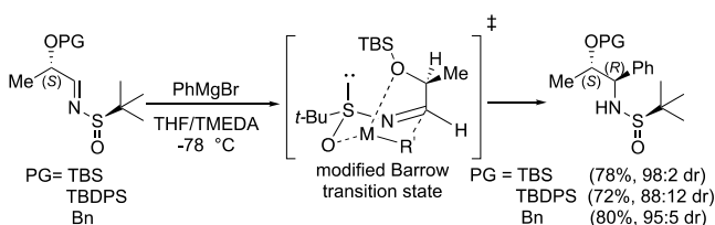
Figure 4. Influence of protecting group on diastereoselectivity and yield.
