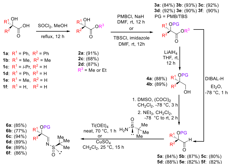
Scheme 6. General Routes for the Synthesis of \alpha -Siloxy Sulfinimines from Hydroxy Acids and Esters
