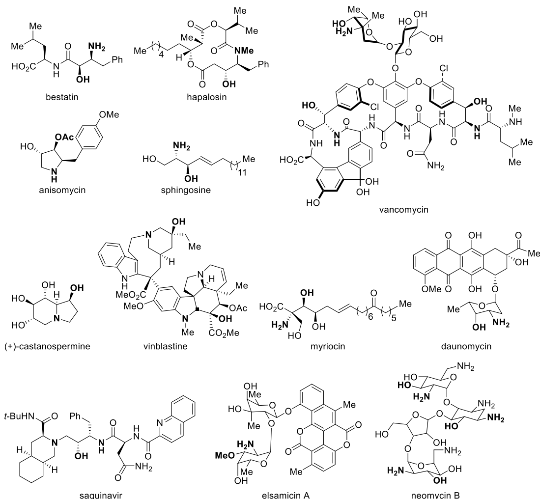
Chart 1. Selected Examples of Natural Products and Pharmaceutically Active Compounds with 1,2-Amino Alcohol Motifs
