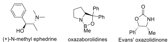
Figure 1. Examples of 1,2-amino alcohol-containing chiral auxiliaries.
