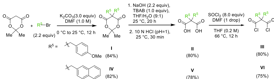
Scheme 7. Preparation of Malonyl Dichlorides with Various Bridging Substituents
