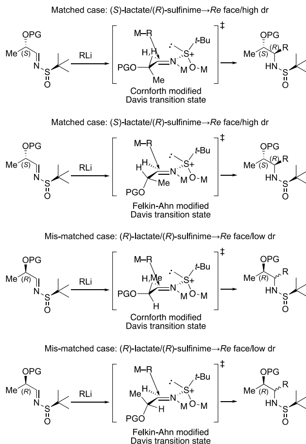
Figure 5. Modified Davis models for matched and mismatched additions.
