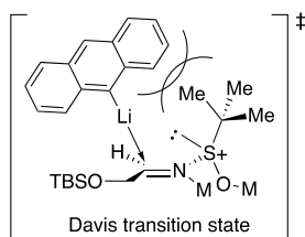
Figure 6. Origin of decreased selectivity in addition to 6f with bulky nucleophiles.
