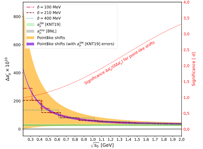
FIG. 6. Energy-dependent decreases \Delta a'_\mu from adjustments to \sigma_{\text{had}}(s) to account for \Delta[\Delta\alpha_{\text{had}}^{(5)}(M_Z^2)] = -3.9(4.3) \times 10^{-4} . The dashed-crimson, dashed-maroon, and dashed-cyan lines represent the binned shifts for \delta = 100, 210, 400 MeV, respectively. The orange band defines the uncertainty for the curve obtained for pointlike increases \Delta b(\sqrt{s_0}) . The purple band shows the central values of \Delta a'_\mu , but with \Delta a in each case forced to have the same precision as a_\mu^{\text{SM}} [KNT19]. The KNT19 result \Delta a_\mu = (28.0 \pm 7.4) \times 10^{-10} is given by the light-green band [23]. The experimental measurement of a_\mu [2–5], corresponding to \Delta a_\mu = 0 , is given by the gray band. The dashed-red line, corresponding to the right-hand y axis only, shows the significance in standard deviations of the difference between a_\mu^{\text{exp}} and the orange band.
