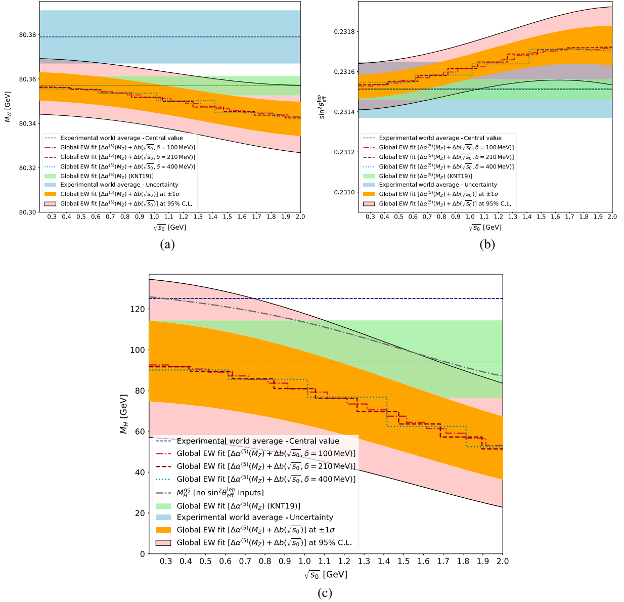
FIG. 2. The values of M_W , \sin^2 \theta_{\text{eff}}^{\text{lep}} , and M_H obtained from the GFITTER global EW fit using as input the increased values of \Delta\alpha_{\text{had}}^{(5)}(M_Z^2) + \Delta b shown in Fig. 1. (a) The W boson mass, M_W . (b) The effective weak mixing angle, \sin^2 \theta_{\text{eff}}^{\text{lep}} . (c) The Higgs boson mass, M_H . The orange band displays the curve obtained for pointlike increases \Delta b(\sqrt{s_0}) , where the width of the band is the \pm 1\sigma uncertainty obtained from the fit (including both parametric and theoretical errors). The solid black lines outlining the pink band indicate the upper/lower bounds of the EW observable determined from the fit at the 95% C.L. The dashed-crimson, dashed-maroon, and dashed-cyan lines represent the value obtained from binned shifts \Delta b(\sqrt{s_0}, \delta) for \delta = 100, 210, 400 MeV, respectively. The result for each observable determined from the EW fit using the KNT19 result for \Delta\alpha_{\text{had}}^{(5)}(M_Z^2) is given by the light-green band. The dashed-navy line indicates the central value of the measured value of each EW observable, the uncertainty of which is displayed by the light-blue band. The gray dash-dotted line in (c) indicates GFITTER's prediction for the 95% C.L. upper bound on M_H obtained omitting all the measurements which lead to the present \sin^2 \theta_{\text{eff}}^{\text{lep}} experimental average from Z-pole measurements (see Sec. II C).
