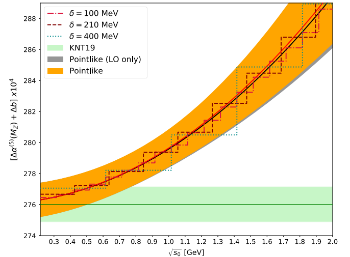
FIG. 1. Energy-dependent increases \Delta\alpha_{\text{had}}^{(5)}(M_Z^2) + \Delta b obtained when adjusting \sigma_{\text{had}}(s) to account for \Delta a_\mu . The dashed-crimson, dashed-maroon, and dashed-cyan lines represent the binned shifts \Delta b(\sqrt{s_0}, \delta) for \delta = 100, 210, 400 MeV, respectively. The solid red line displays the curve obtained for pointlike increases \Delta b(\sqrt{s_0}) , with the uncertainty given by the orange band. For a comparison of the result obtained in [7], the solid black line and gray band show the result obtained when f(s) accounts for only the LO contributions to a_\mu^{\text{had,VP}} . The KNT19 result for \Delta\alpha_{\text{had}}^{(5)}(M_Z^2) is given by the light-green band [23].
