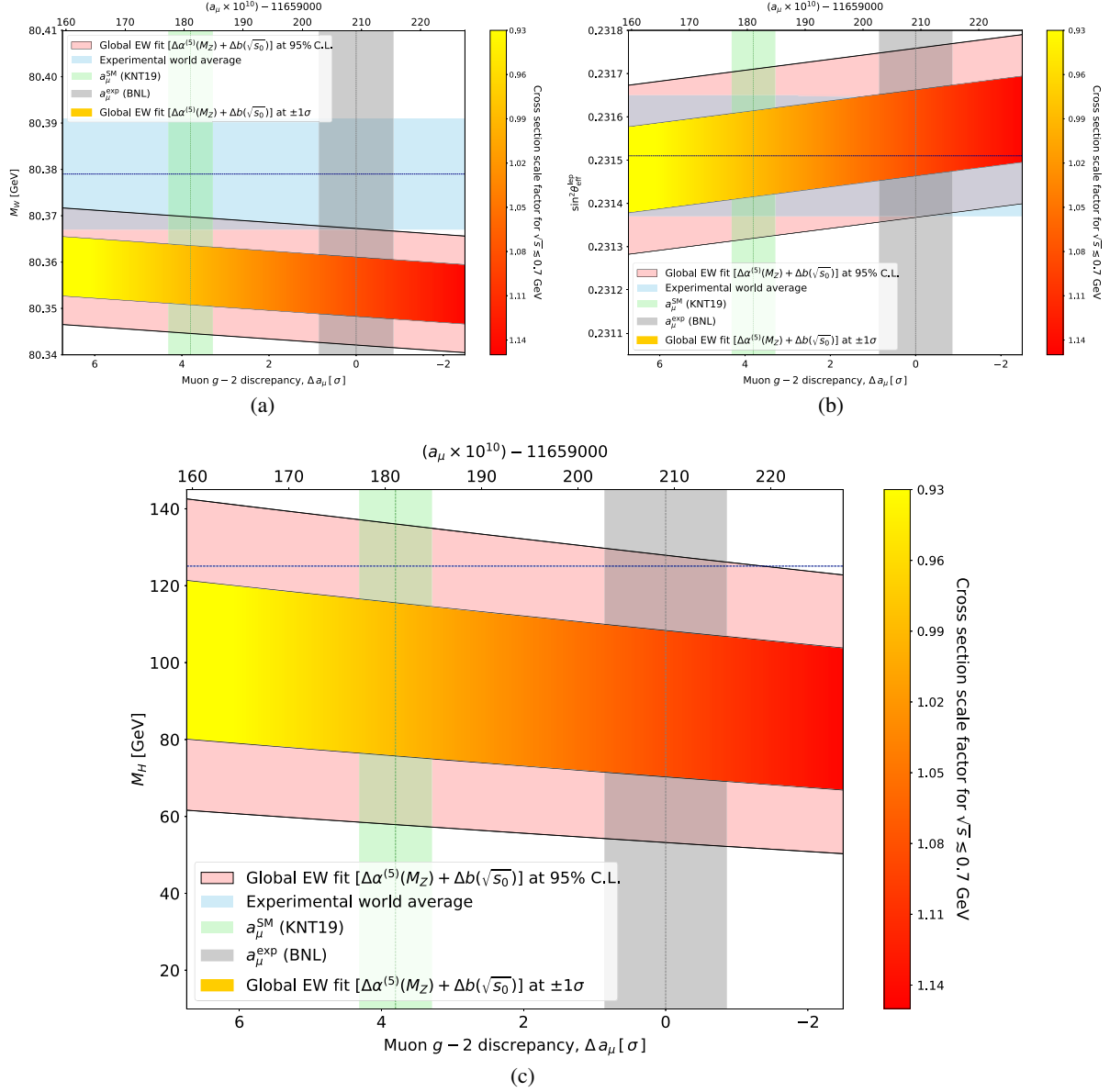
FIG. 3. Plots of M_W , \sin^2 \theta_{\text{eff}}^{\text{lep}} , and M_H vs a_\mu and the resulting muon g-2 discrepancy \Delta a_\mu [\sigma] obtained when scaling \sigma_{\text{had}}(s) in a single energy-independent region \sqrt{s} \lesssim 0.7 GeV. (a) The W boson mass, M_W . (b) The effective weak mixing angle, \sin^2 \theta_{\text{eff}}^{\text{lep}} . (c) The Higgs boson mass, M_H . In each case, the graded yellow-red band displays the value of each observable obtained from the GFITTER global EW fit, using as input the shifted values of \Delta\alpha_{\text{had}}^{(5)}(M_Z^2) determined from the scaled \sigma_{\text{had}}(s) . The width of this band is the \pm 1\sigma uncertainty obtained from the fit (including both parametric and theoretical errors). The yellow-red color gradient of this band and the z axis indicates the magnitude of the scale factor \epsilon that is applied to account for \Delta a_\mu . The solid black lines outlining the pink band indicate the upper/lower bounds of the EW observable determined from the fit at the 95% C.L. The light-blue band indicates the measured value of each EW observable. The KNT19 result for a_\mu^{\text{SM}} is given by the light-green band, corresponding to \Delta a_\mu = 3.8\sigma [23]. The experimental measurement of a_\mu [2–5], indicating a no-new-physics scenario and corresponding to \Delta a_\mu = 0 , is given by the gray band.
