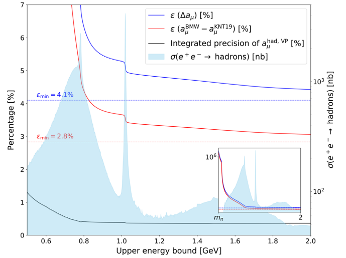
FIG. 5. The increase of \epsilon (%) required to account for the muon g-2 discrepancy (solid blue line), as well as the discrepancy between the lattice BMW [85] and dispersive KNT19 results [23] (solid red line), when adjusting \sigma_{\text{had}}(s) from threshold up to a given upper energy bound. The dashed-blue and dashed-red lines show the minimum increase required (corresponding to an upper energy bound of \infty ) for \Delta a_\mu and the lattice BMW vs dispersive KNT19 evaluations, respectively. The solid black line depicts the precision in percentage of a_\mu^{\text{had,VP}} when integrating from threshold to the upper energy bound. The total e^+e^- \rightarrow \text{hadrons} cross section is given by the light-blue shaded region for reference.
