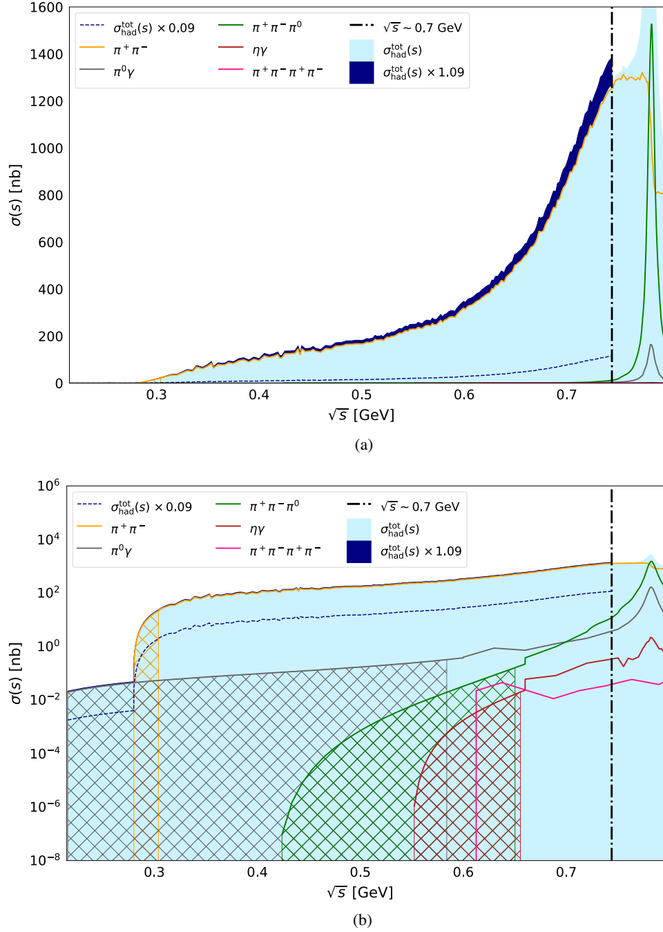
FIG. 4. Contributions to the total hadronic cross section from the hadronic modes contributing below \sim 0.7 GeV, plotted (a) for a linear y axis and (b) for the y axis represented on a log scale. The total cross section is shown by the filled light-blue region in each plot. The vertical dashed-black line indicates the exact point at \sqrt{s} \sim 0.7 GeV below which the navy-blue dashed line displays the \epsilon = +9\% shift of the cross section that is applied to account for \Delta a_\mu . The applied increase of \epsilon = +9\% to the total cross section is given by the filled navy area. For each of the hadronic modes, the crosshatched pattern indicates the portion of that hadronic mode that is estimated from ChPT (plus \omega dominance for the \pi^+\pi^-\pi^0 and \pi^0\gamma channels) [61] due to a lack of experimental data at threshold.
