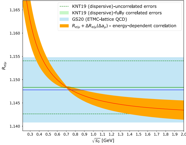
FIG. 8. R_{e/\mu} obtained when adjusting \sigma_{\text{had}}(s) to account for \Delta a_\mu . The solid red line displays the curve obtained for pointlike increases, with the uncertainty given by the orange band. The result determined from the KNT19 values result is given by the light-green band (for 100% correlated errors from e and \mu ) and the dashed-green lines (for uncorrelated errors from e and \mu ). The light-blue band shows the recent lattice QCD evaluation of [122].
