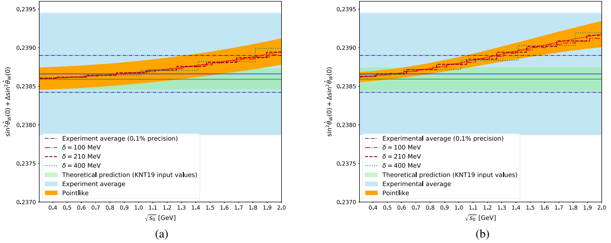
FIG. 9. Predictions for \sin^2 \hat{\theta}_W(0) obtained adjusting \sigma_{\text{had}}(s) to account for \Delta a_\mu . (a) Scenario (1), where the experimental measurement for \sin^2 \theta_{\text{eff}}^{\text{lep}} is used as input into Eq. (3.7). (b) Scenario (2), where the varied values of \sin^2 \theta_{\text{eff}}^{\text{lep}} predicted from the EW fit are used as input into Eq. (3.7). The solid red line displays the curve obtained for pointlike increases, with the \pm 1\sigma uncertainty given by the orange band. The dashed-crimson, dashed-maroon, and dashed-cyan lines represent the binned shifts for \delta = 100, 210, 400 MeV, respectively. The theoretical prediction corresponding to KNT19 input values is given by the light-green band [23]. The experimental average of \sin^2 \hat{\theta}_W(0) obtained in Table IV is given by the light-blue band. The navy-blue bands depict the expected future uncertainty on the measured value [134,135].
