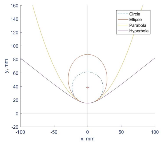
Fig. 11 Example of conic sections with the same latus rectum ( p = 23.1194 mm). Notes: numerical eccentricity of ellipse, e = 0.6 and numerical eccentricity of hyperbola, e = 1.5946 .
