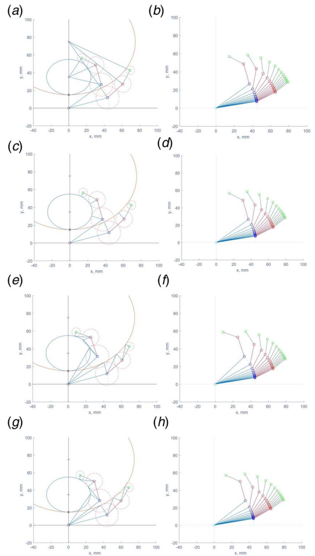
Fig. 5 Numerical simulation example for an object with an elliptic cross section ( a > b ). Notes: First column, an example of the finger motion for each corresponding contact method; second column, the simulated stepwise motion of finger joints (displayed for different values of the control parameter associated with the conic section under consideration).
