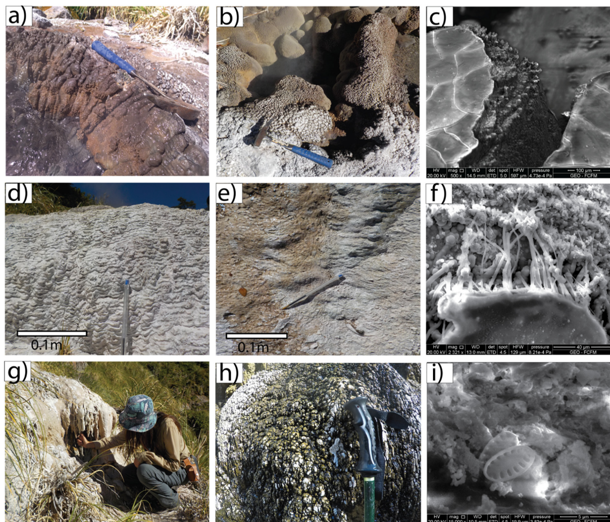
Fig. 5. Proximal deposit or geyserites: (a) columnar texture of a perpetual spouter, (b) spicular texture in geyser splash zone, (c) SEM image of desiccation cracks overlapping microspicules. Mid environment: (d) micro terraces, (e) streamer fabric, (f) SEM image of microbial filaments. Distal environment: (g) sinter stalactites and plants being covered by sinter, (h) secondary splash texture (geyserite-like), and (i) SEM image of diatoms incorporated into the sinter.
