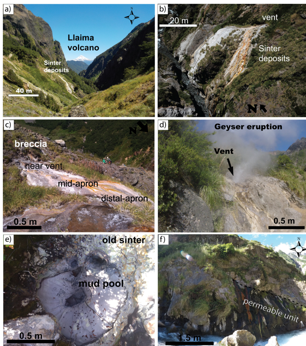
Fig. 3. (a) Panoramic view of Alpehuevo canyon looking north toward the Llama volcano (Fig. 1a), (b) UAV view of sinter deposits looking at site 3, (c) sinter deposit laying on breccia at site 4, (d) geyser eruption at site 2, (e) mud pool breaking old sinter at site 5, and (f) hot spring in the river at site 8.
