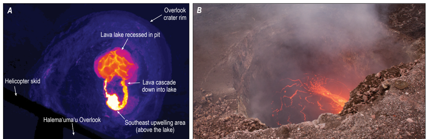
Figure 33. Photographs taken after the Kamoamo eruptive event of March 2011, when the summit reinflated and the lava lake refilled. A, In May, the lava lake was often recessed in a pit. Occasionally, lava upwelled from a spot southeast of the lake, sending two lava streams cascading downward into the lake. Thermal image taken on May 11, 2011, by Matt Patrick using a FLIR SC620 camera. Purple and black colors represent cool temperatures, yellow and white colors represent hot temperatures. B, Lava pours from a vent in the south part of the crater and flows northward in a channel. The lake continued refilling until early August 2011, when it drained again during another East Rift Zone eruptive event. Photograph taken on June 2, 2011, from the Halema'uma'u rim by Ben Gaddis, Hawaiian Volcano Observatory volunteer.
