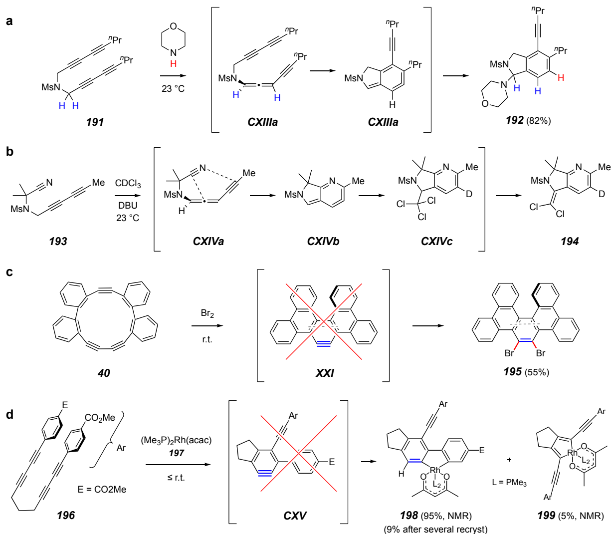
Figure 23. Reactions of polyyne substrates that proceed under conditions that would not promote appreciable levels of HDDA benzyne, indicating that the co-reactant is promoting cyclization by engaging the substrate prior to the thermal HDDA cycloisomerization.
