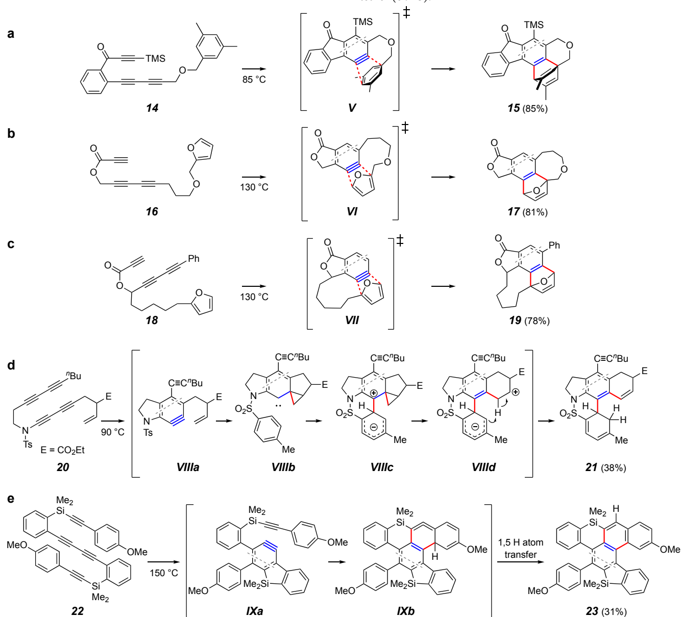
Figure 4. Intramolecular traps forming two C–C bonds.
