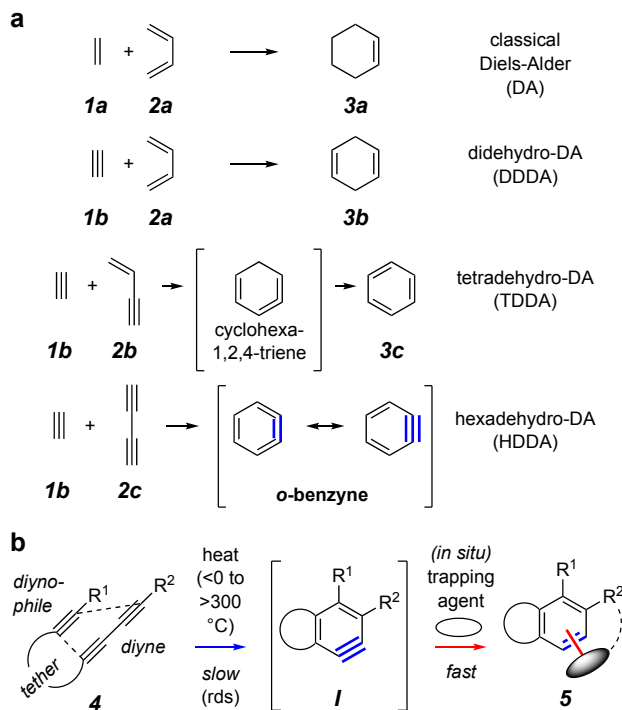
Figure 1. (a) The family of prototypical classical and various dehydro-Diels-Alder reactions of increasing oxidation states. (b) The generic intramolecular hexadehydro-Diels-Alder (HDDA) cyclization and benzyne-trapping reaction.
