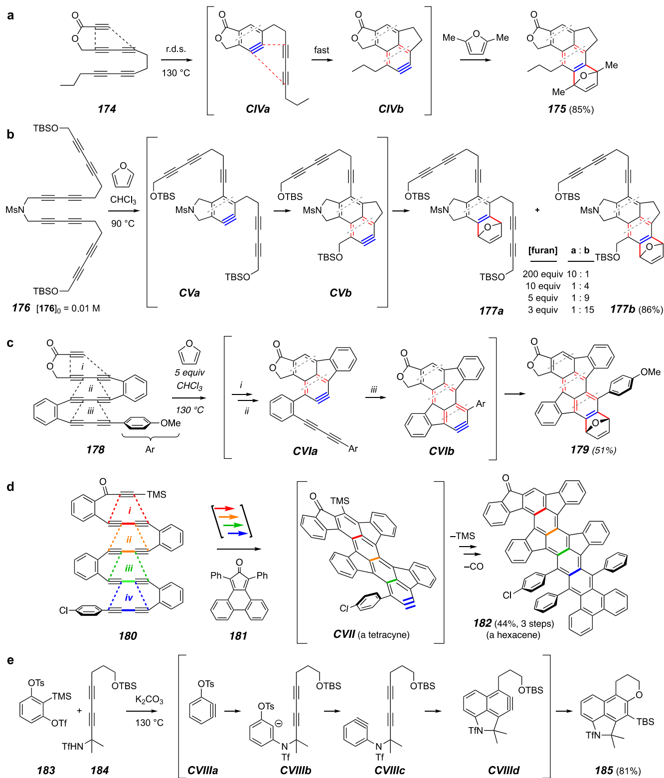
Figure 21. Examples of the domino HDDA reaction. (a) Benzyne to naphthylene. (b) Evidence for the intermediacy of a benzyne. (c) Benzyne to naphthylene to anthracene. (d) Benzyne to naphthylene to anthracene to tetracyne. (e) A domino cascade involving benzyne generated by both classical and HDDA processes.
