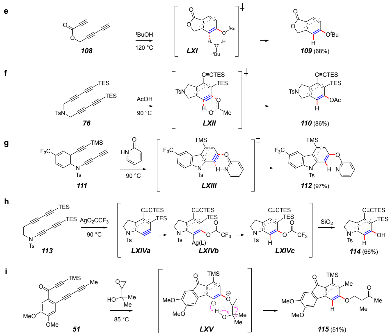
Figure 12 (cont. from previous page). Trapping reactions forming a C–O and a C–H bond.
