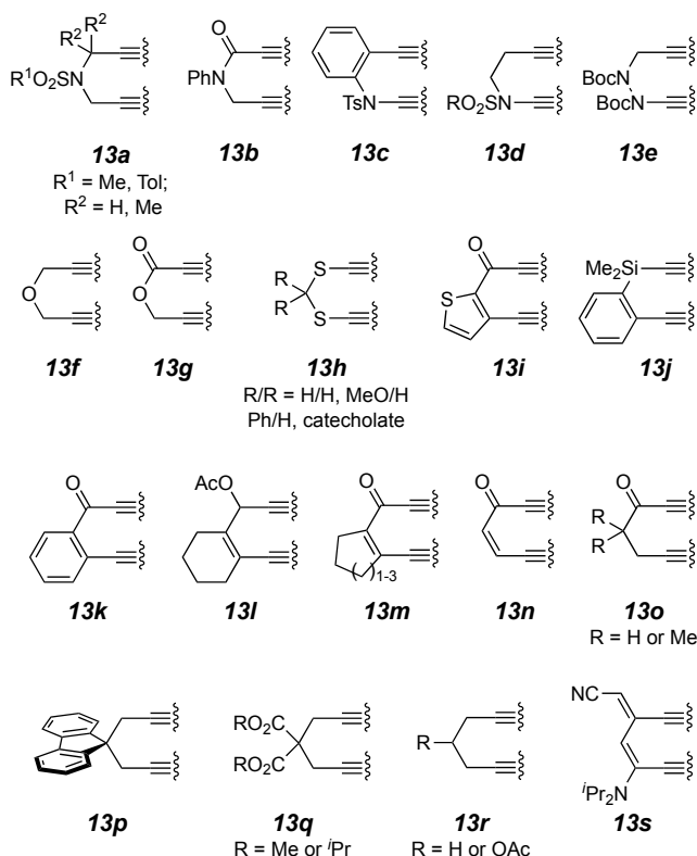
Figure 3. The majority of the three-atom tethers present in reported HDDA polyynes.
