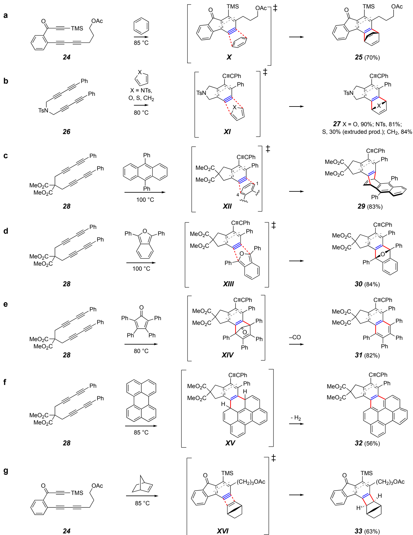
Figure 5. (cont. on next page)
