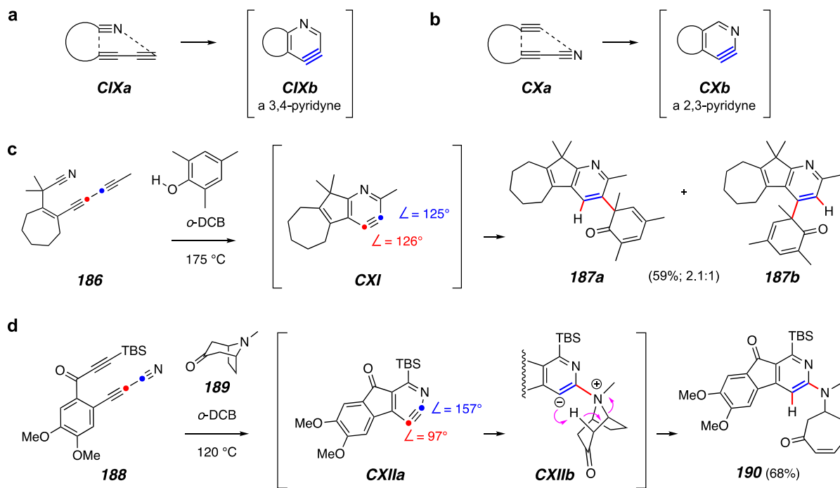
Figure 22. Aza-HDDA reactions. (a) Generic formation of a 3,4-pyridyne. (b) Generic formation of a 2,3-pyridyne. (c) A relatively unselective trapping of a 3,4-pyridyne. (d) A highly selective trapping of a 2,3-pyridyne.
