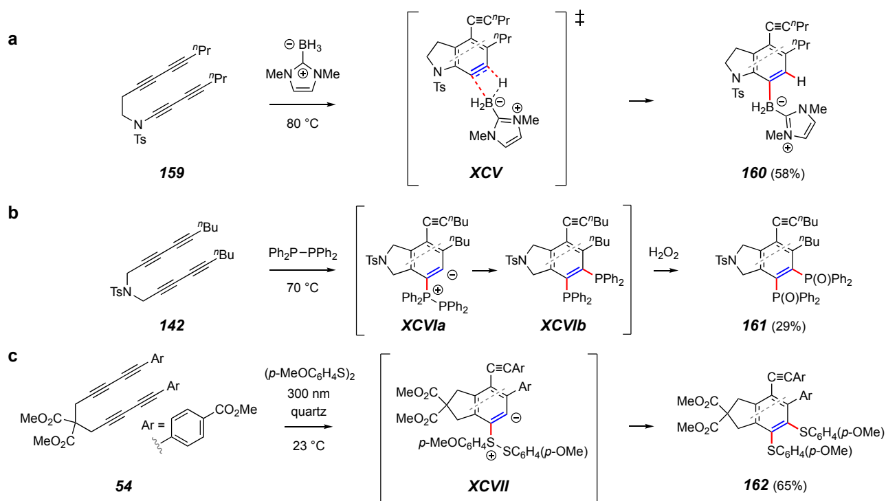
Figure 19. Trapping reactions that form (a) a C–H and a C–B bond, (b) two C–P bonds, and (c) two C–S bonds.
