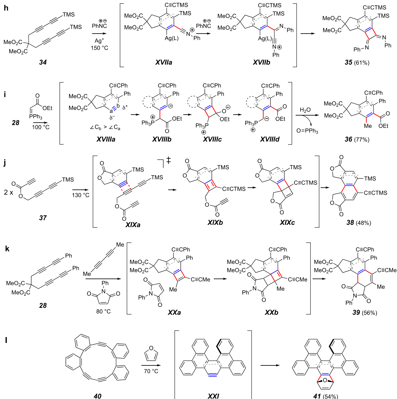
Figure 5 (cont. from previous page). Intermolecular traps forming two C–C bonds.
