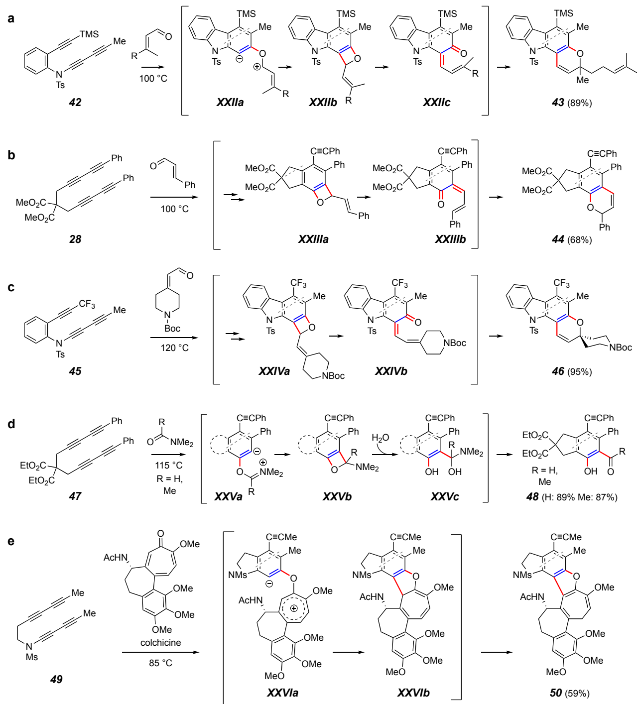
Figure 6. Trapping reactions forming a C–C and a C–O bond. (a–c) Reactions with enals begins with benzoxetene formation prior to electrocyclic opening and reclosure to produce benzopyrans. (d) Nucleophilic amides capture benzynes to product o -hydroxy aldehydes and ketones such as 48 . (e) The cycloheptatrienone in colchicine captures an HDDA-produced benzyne to give the benzofuran derivative 50 .
