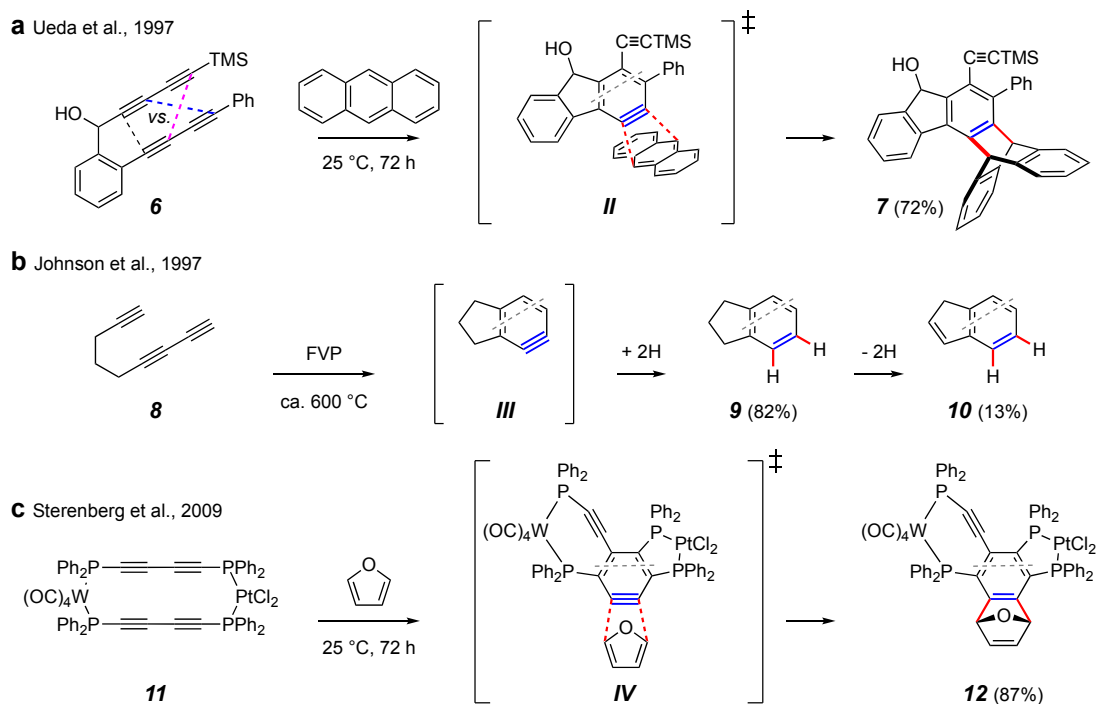
Figure 2. Earliest reports of cyclization of a triyne to a benzyne intermediate. (a) Ueda and coworkers (1997): trapping of the benzyne II with anthracene gives the triptycene 7 . (b) Johnson and coworkers (1997): high temperature (short time) cycloisomerization of 8 to 10 via III and 9 . (c) Sterenberg and Tsui (2009): intra-annular cyclization of dinuclear complex 11 in the presence of furan gives the adduct 12 via IV .
