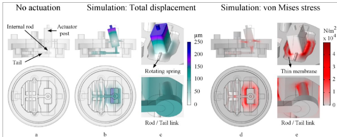
Figure 2. Simulated actuation of the proposed system. The top panels show side views, and the bottom panels show bottom views. Column (a) shows the assembly without actuation. Column (b,c) show the simulated total displacement ( \mu\text{m} ) under actuation, where (c, top) is a top isometric view of the actuator post, and (c, bottom) is a bottom isometric view of the rod, and tail link. Column (d,e) show the simulated von Mises stress ( \text{N/m}^2 ), where (e, top) is a top isometric view of the actuator post, and (e, bottom) is a bottom isometric view of the rod and tail link.
