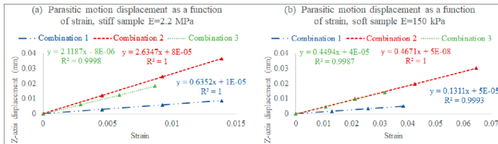
Figure 6. Simulated assembly combination examples showing the strain vs. parasitic displacement relationships (at the sample level) for (a) a stiff sample with an elastic modulus of E = 2.2 MPa, and (b) a soft sample with an elastic modulus of E = 150 kPa (simulated at fixed sample dimensions and forces). Legends: Combination 1, a stiff lid (3 MPa) and a stiff stage (3 MPa); Combination 2, a soft lid (850 kPa) and a soft stage (850 kPa); and Combination 3, a stiff lid (3 MPa) and a soft stage (850 kPa) (the assembly combinations with the least sample parasitic motion and highest actuator strain and sensor sensitivity for the targeted sample stiffness were chosen for testing).
