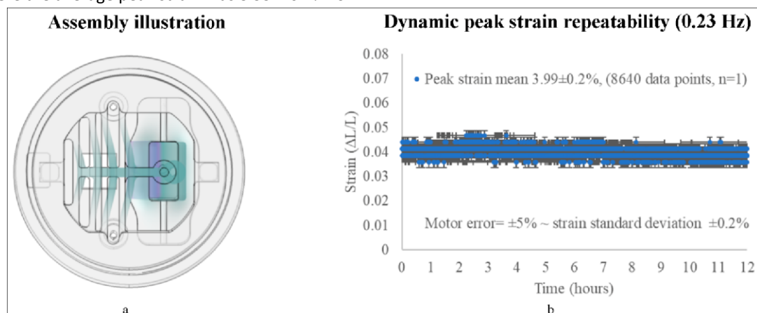
Figure 10. PDMS assembly stretching mechanism with a PDMS monolayer attached and sensor engaged, where (a) is a simulation/illustration of the stretching mechanism and (b) is the dynamic strain repeatability for 12 h at 0.23 Hz (8640 high peak data points); n = 1 . Measured data are presented as the mean \pm standard deviation (error bars).
