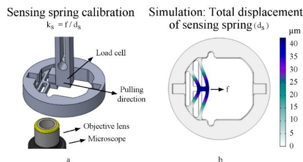
Figure 5. Sensor calibration, where (a) is an illustration of the measurement and (b) is the matching simulation.
