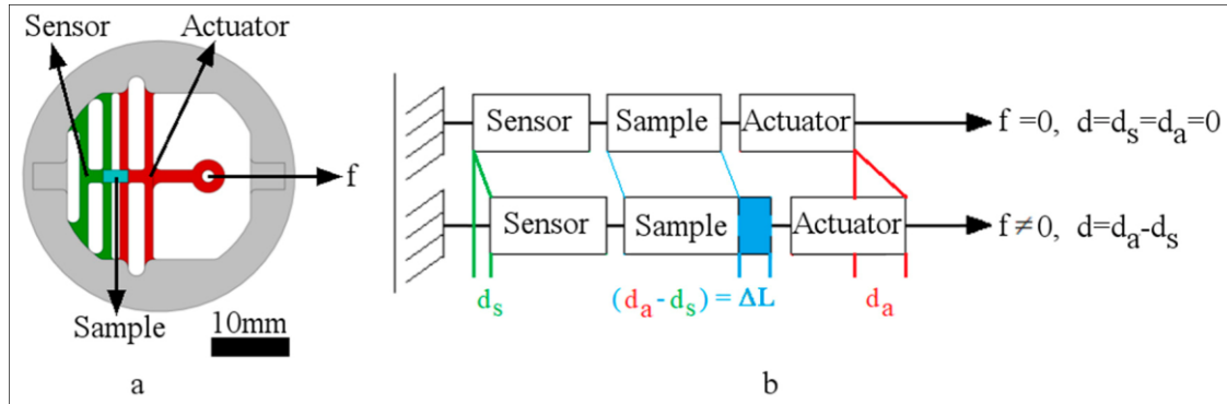
Figure 3. (a) Colored stage parts representing (b) a schematic diagram of the stage theory of operation (non-actuated vs. actuated) (the actuator is shown in red, the sample in blue, and the sensor in green). Scale bar = 10 mm.
