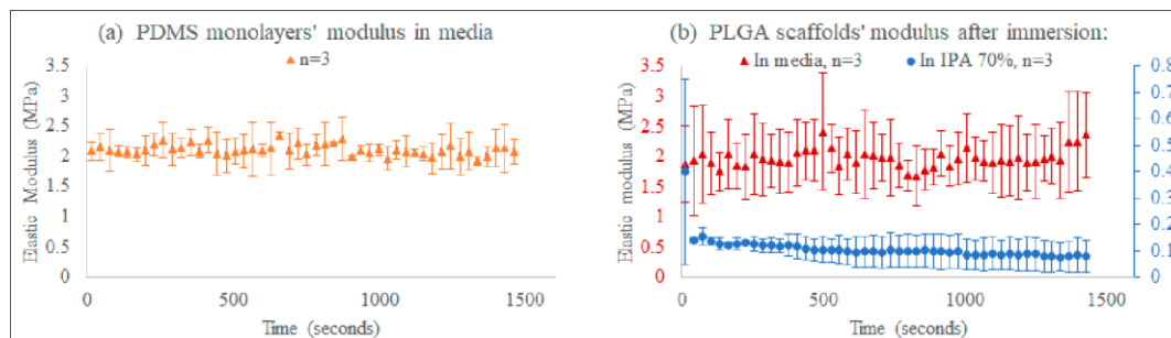
Figure 14. Time-course mechanical characterization of (a) stiff PDMS sheets in media (shown in orange, n = 3 ), and (b) PLGA 85:15 film in media (shown in red, n = 3 ) and in IPA 70% (shown in blue, n = 3 ). Measured data are presented as the mean \pm standard deviation (error bars).
