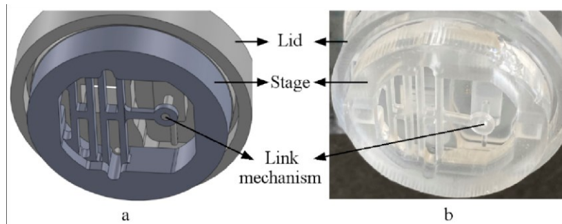
Figure 9. A bottom isometric view of the uniaxial assembled system: (a) SolidWorks design and (b) actual cured PDMS, showing the tail/rod link mechanism (no sample attached).
