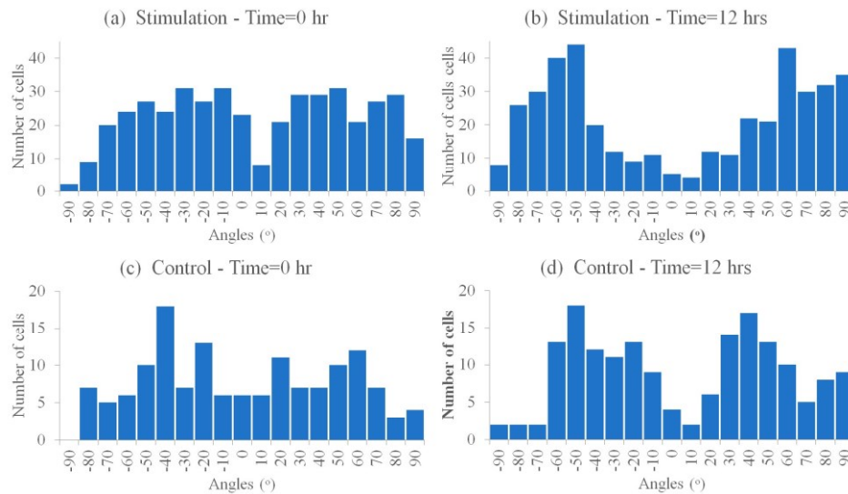
Figure 15. Histograms showing cells' angle distribution, where (a) is the stimulation at t = 0 h, cells# 429; (b) is the stimulation at t = 12 h, cells# 415; (c) is the control at t = 0 h, cells# 145; and (d) is the control at t = 12 h, cells# 170 (cell angle data were pooled from stimulated samples, n = 3 , and from control samples, n = 2 ).
