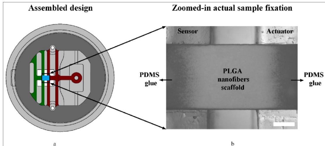
Figure 8. Sample attachment to springs using PDMS as glue: (a) shows the assembled design, where the sample is shown in blue, while (b) is a zoomed-in image of an actual PDMS-glued specimen (electrospun PLGA 85:15 nanofiber film > 6-months-old). Scale bar = 50 \mu\text{m} .
