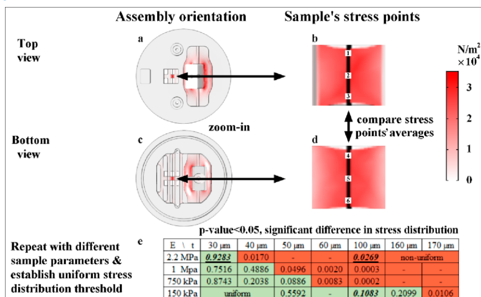
Figure 7. The uniform stress distribution threshold across samples, based on their elastic moduli (E) and thicknesses (t), ( n = 1 for each simulation thickness and modulus); (a) is a top view of the computational analysis (COMSOL); (b) is a zoomed-in snapshot of the sample's top side stress points; (c) is a bottom view of the
