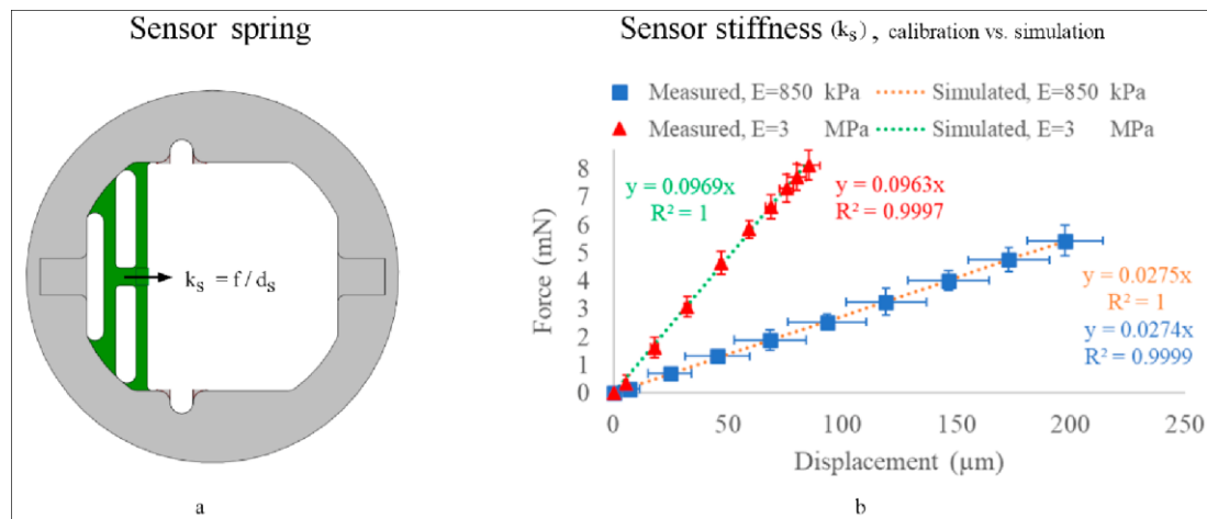
Figure 11. Calibration of sensing spring constants ( k_s ). (a) is an illustration, while (b) is the measured sensing spring constants vs. simulated ones, with n = 5 for each fabrication condition. The simulated stiffness equation for fabrication condition 1 (in green) is y = 0.0969x ( R^2 = 1 ), and the measured value (shown in red) is y = 0.0963 ( R^2 = 0.9997 ). The simulated stiffness equation for fabrication condition 2 (in orange) is y = 0.0275x ( R^2 = 1 ), and the measured value (shown in blue) is y = 0.0274x ( R^2 = 0.9999 ). Measured data are presented as the mean \pm standard deviation (error bars).
