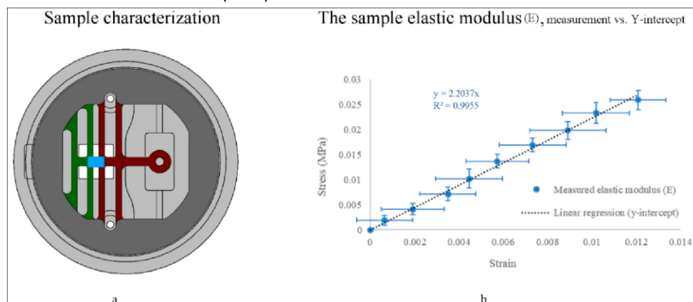
Figure 13. PDMS specimen Young's modulus E characterization. (a) is an illustration (sample shown in blue), and (b) is an end-point measurement of a spin-coated PDMS sample ( E = 2.2 MPa) (blue, n = 9 ) vs. linear regression (in black). The elastic modulus equation for the linear regression is y = 2.2037x , R^2 = 0.9955 . Measured data are presented as the mean \pm standard deviation (error bars).
