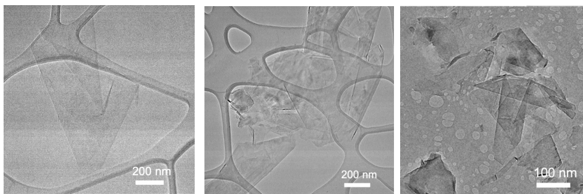
Figure S4. TEM images of the top fraction of the exfoliated graphite, which were cleaved off from larger graphite particles. The background is lacey carbon (400 mesh grid).
