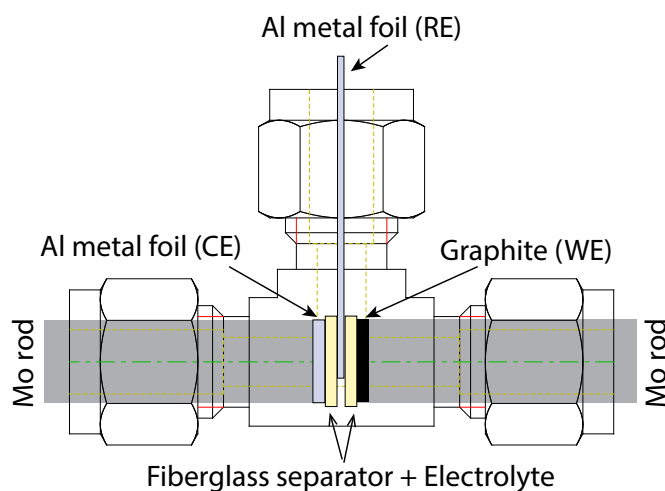
Figure S2. Three-electrode cell geometry used for EIS measurements.
