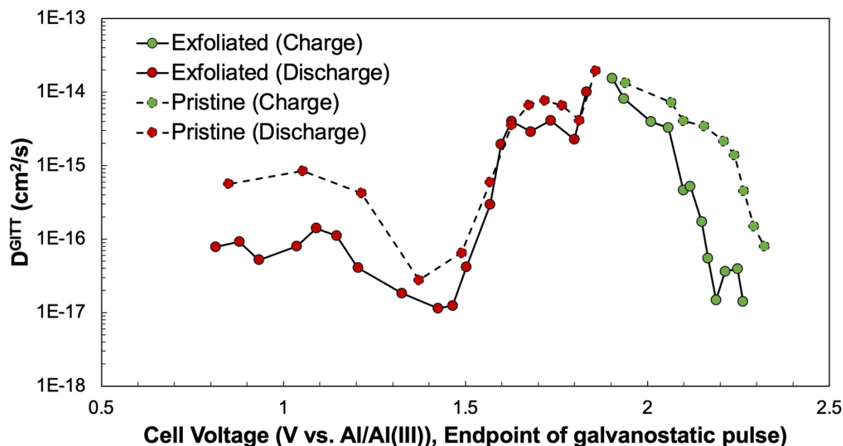
Figure S8. Apparent ionic diffusion coefficients estimated by GITT ( D^{\text{GITT}} ), as a function of cell potential, for pristine and exfoliated graphite cells. See Text S1 for a more detailed analysis, including the underlying assumptions and why GITT analyses are not accurate for rechargeable Al-graphite cells.
