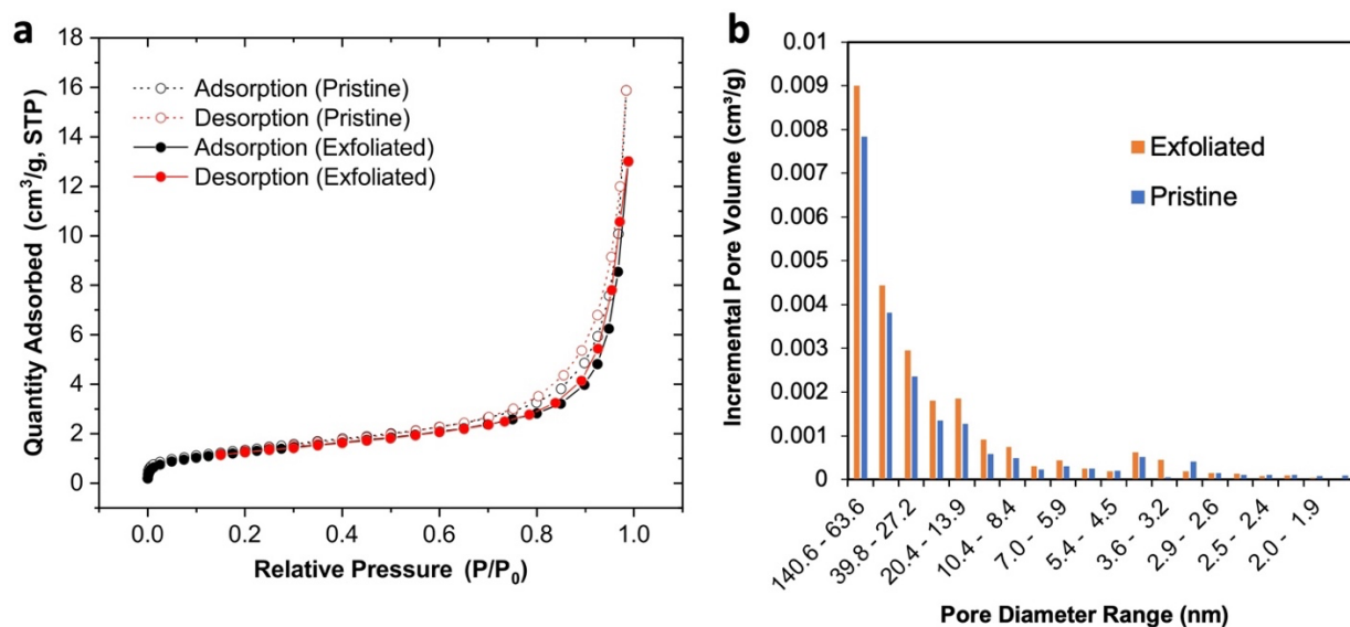
Figure S5. (a) N 2 sorption isotherm for exfoliated and pristine graphite particles before incorporation into a composite electrode. The pristine graphite was soaked in NMP for 2 h and vacuum dried overnight, but not ultrasonicated, to subject it to an otherwise similar preparation process. (b) BJH pore size distributions for exfoliated and pristine graphite.
