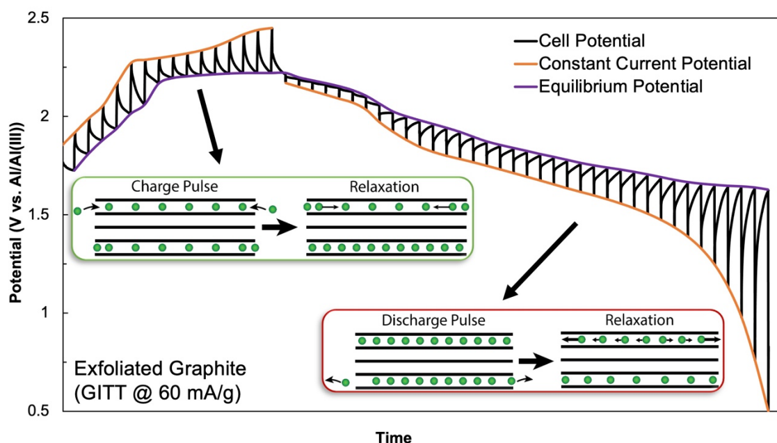
Figure S7. Representative GITT test performed on a two-electrode Al-graphite cell containing exfoliated graphite.
