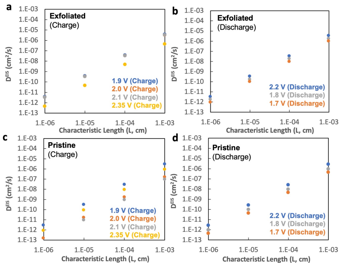
Figure S9. The dependence of the diffusion coefficients determined by EIS ( D_{\text{EIS}} ), calculated using a modified Warburg element, with different characteristic diffusion lengths ( L ) for (a-b) exfoliated and (c-d) pristine graphites.
