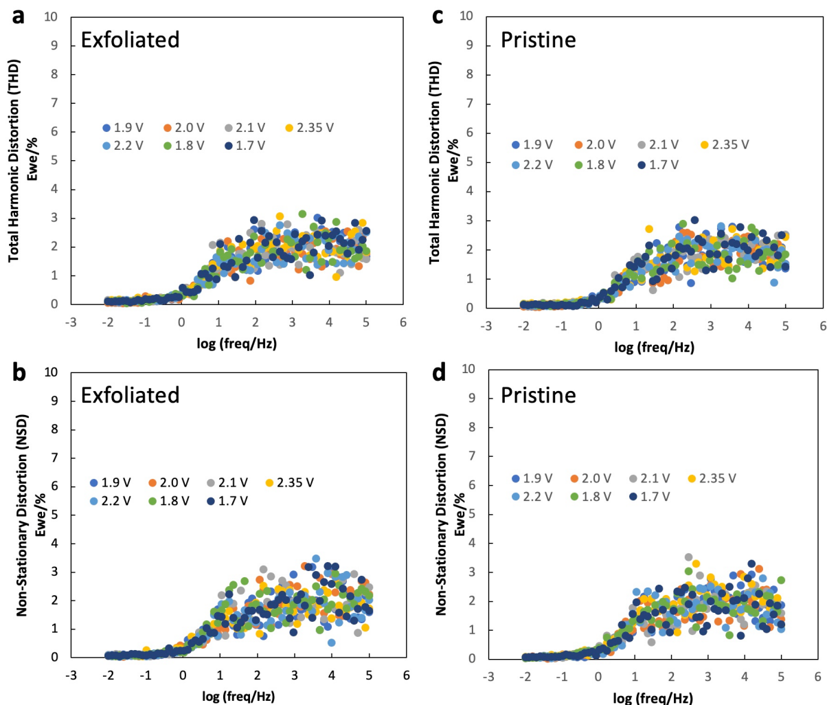
Figure S3. Total Harmonic Distortion (THD) and the Non-Stationary Distortion (NSD) analyses of the electrochemical impedance spectroscopy data for Al-graphite cells containing exfoliated (a-b) and pristine (c-d) graphite electrodes.
