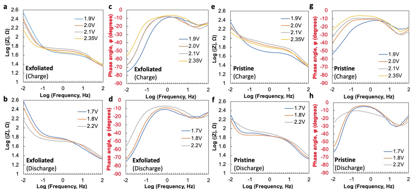
Figure S6. Bode plots of EIS data for Al-graphite cells containing (a-d) exfoliated graphite and (e-h) pristine graphite cycled to different potentials, showing the dependance of the (a,b,e,f) overall impedance Z and (c,d,g,h) phase angle \phi as a function of frequency.
