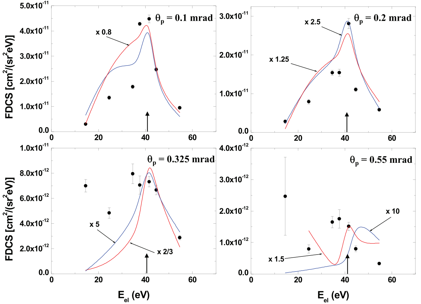
FIG. 7. Same as Fig. 3, but for electron ejection from H_2 .
