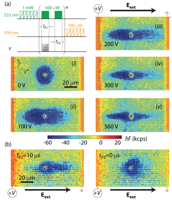
FIG. 3. \tilde{\tau}_E = n(t_{\text{p1}} + t_{\text{p2}}) Charge dynamics in the presence of pulsed electric fields. (a) Experimental protocol (top left); the total parking time amounts to t_{\text{p1}} + t_{\text{p2}} . [(i)–(v)] Differential NV - fluorescence maps for different applied voltages; in these experiments, t_{\text{p1}} = 1 \text{ ms} , t_{\text{p2}} = 1 \text{ ms} , \tilde{\tau}_P = 1 \text{ min} , and the arrow denotes the direction of the externally applied electric field. (b) (Left) Same as above but for t_{\text{p2}} = 10 \mu\text{s} (right) or t_{\text{p2}} = 0 \mu\text{s} (left) at 420 V. The same color bar applies to both (a) and (b).
