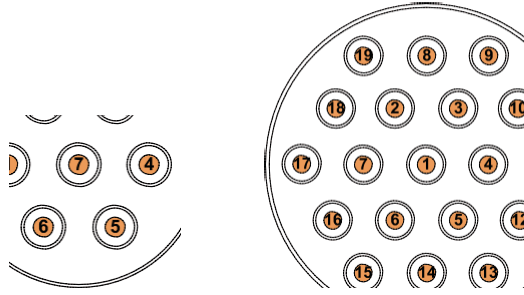
Fig. 9. Test MCFs.
