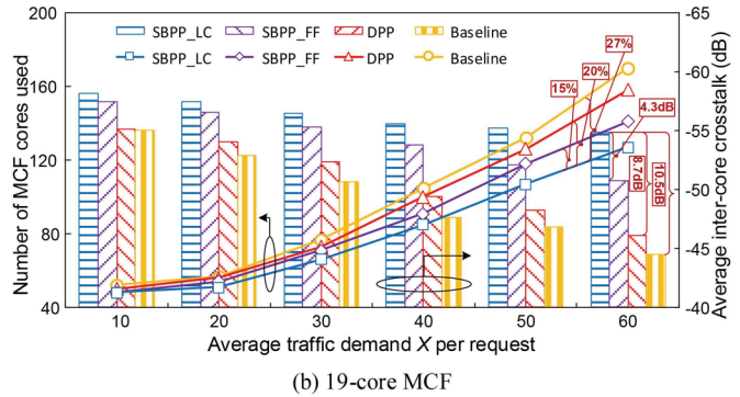
Fig. 11. Performance comparison in terms of the number of cores used and average inter-core crosstalk (COST239).
