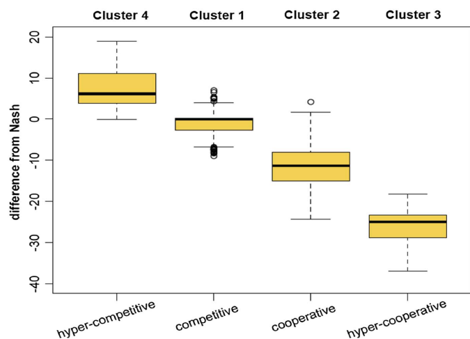
Fig. 2. Box plots of differences to Nash equilibria for the four behavioral groups.
