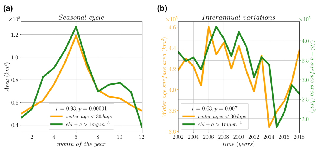
Figure 2. Area occupied by high Chl-a events ( >1 \text{ mg m}^{-3} , green line, right axis) and area occupied by young water age events ( <30 days, orange line, left axis). (a) Mean seasonal cycle ( r = 0.93 ; p < 0.01 between the two signals) and (b) interannual variability ( r = 0.63 ; p < 0.01 between the two signals). Averaged between 30^\circ and 40^\circ\text{N} .
