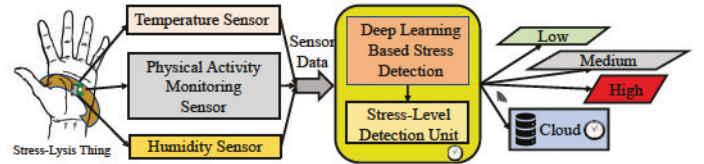
Fig. 1. The proposed architecture of the Stress-Lysis system [1].
