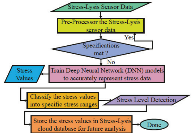
Fig. 2. The proposed algorithm for stress detection in Stress-Lysis [1].
