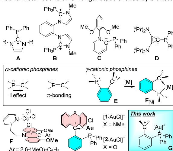
Fig. 1. Top: The carbenium resonance form of arbitrarily selected examples of \alpha -cationic phosphines. Inset: possible electronic effects at play in \alpha - and \gamma -cationic phosphines. Bottom: Recently isolated examples of complexes pendent carbenium units and dicationic complexes targeted in this study.
