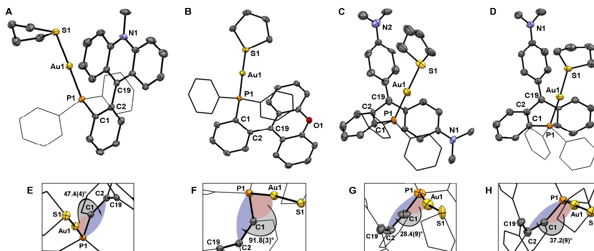
Fig 5. ORTEP representations of the structures of [1-Au(tht)][BF 4 ] 2 (A), [2-Au(tht)][BF 4 ] 2 (B), [3-Au(tht)][BF 4 ] 2 (C), and [4-Au(tht)][BF 4 ] 2 (D), with a close up showing the torsion angle \alpha_d (E-H). Hydrogen atoms and BF 4 - counterions omitted for clarity. Thermal ellipsoids drawn at 50% probability and phenyl groups drawn as thin lines. Selected bond lengths (Å) and angles (°) for [1-Au(tht)][BF 4 ] 2 : Au(1)-(P1) 2.2699(11), Au(1)-S(1) 2.3352(12), C(19)-C(2) 1.500(6), C(19)-C(20) 1.395(6), C(19)-C(26) 1.406(6); C(2)-C(19)-C(20) 122.1(4), C(20)-C(19)-C(26) 119.6(4), C(26)-C(19)-C(2) 118.3(4). Selected bond lengths (Å) and angles (°) for [2-Au(tht)][BF 4 ] 2 : Au(1)-(P1) 2.2710(9), Au(1)-S(1) 2.3315(9), C(19)-C(2) 1.479(5), C(19)-C(20) 1.414(5), C(19)-C(26) 1.415(4); C(2)-C(19)-C(20) 121.5(3), C(20)-C(19)-C(26) 118.2(3), C(26)-C(19)-C(2) 120.2(3). Selected bond lengths (Å) and angles (°) for [3-Au(tht)][BF 4 ] 2 : Au(1)-(P1) 2.251(5), Au(1)-S(1) 2.286(5), C(19)-C(2) 1.507(19), C(19)-C(20) 1.43(2), C(19)-C(26) 1.43(2); C(2)-C(19)-C(20) 116.3(15), C(20)-C(19)-C(26) 127.5(16), C(26)-C(19)-C(2) 116.2(15). Selected bond lengths (Å) and angles (°) for [4-Au(tht)][BF 4 ] 2 : Au(1)-(P1) 2.281(2), Au(1)-S(1) 2.334(2), C(19)-C(2) 1.477(14), C(19)-C(20) 1.378(14), C(19)-C(26) 1.469(13); C(2)-C(19)-C(20) 120.3(9), C(20)-C(19)-C(26) 121.6(9), C(26)-C(19)-C(2) 117.2(9).
