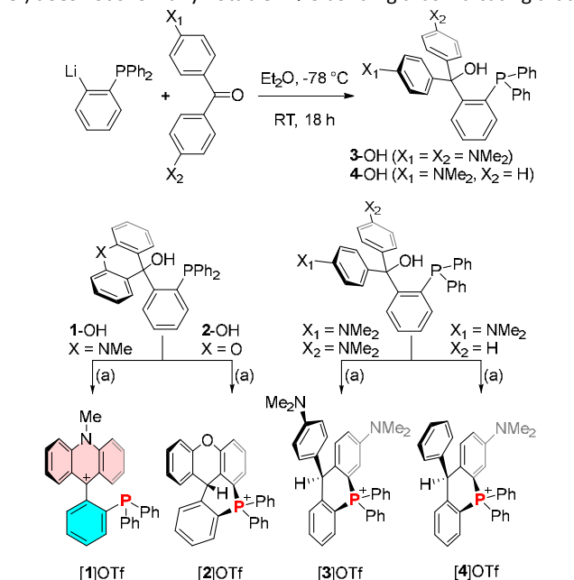
Scheme 1. Top: Synthesis of carbinols 3-OH and 4-OH . Bottom: Synthesis of [1]OTf, [2]OTf, [3]OTf and [4]OTf by dehydroxylation of corresponding carbinols. (a) TMSOTf, CH 2 Cl 2 , RT.
