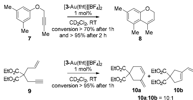
Scheme 5. Intramolecular hydroarylation and enyne cyclization reactions catalyzed by [3\text{-Au}(\text{tht})][\text{BF}_4]_2 .
