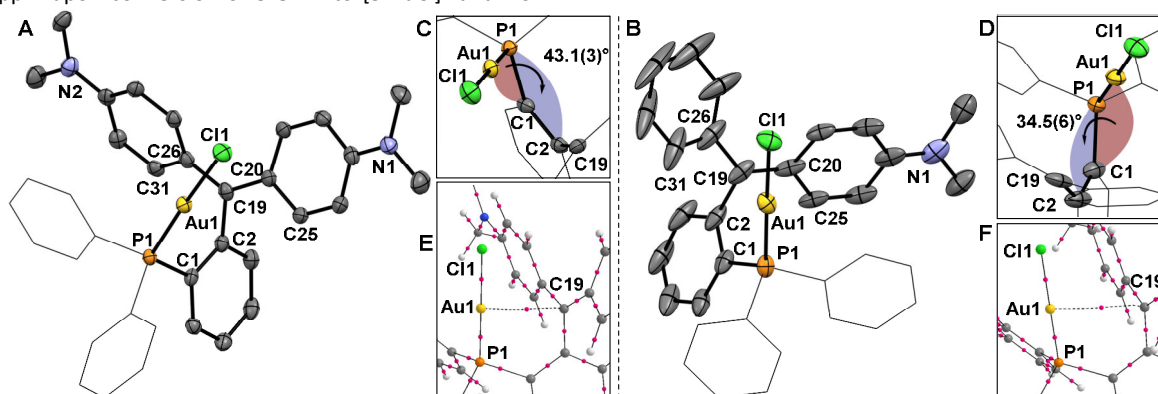
Fig. 4. ORTEP representations of the structures of [3-AuCl][BF 4 ] (A) and [4-AuCl][BF 4 ] (B), with a close up of the torsion angle (C and D). Hydrogen atoms and BF 4 − counterions omitted for clarity. Thermal ellipsoids drawn at 50% probability and phenyl groups drawn as thin lines. Selected bond lengths (Å) and angles (°) for [3-AuCl][BF 4 ]: C(19)–C(2) 1.500(4), C(19)–C(20) 1.413(5), C(19)–C(26) 1.427(5); C(2)–C(19)–C(20) 117.2(3), C(20)–C(19)–C(26) 125.2(3), C(26)–C(19)–C(2) 117.6(3). Selected bond lengths (Å) and angles (°) for [4-AuCl][BF 4 ]: C(19)–C(2) 1.494(11), C(19)–C(20) 1.365(10), C(19)–C(26) 1.473(7); C(2)–C(19)–C(20) 119.0(5), C(20)–C(19)–C(26) 124.8(6), C(26)–C(19)–C(2) 116.1(6). Graphical output of the AIM analysis (E and F) showing the bond critical point between Au1 and C19 at the optimized geometry of [3-AuCl] + and [4-AuCl] + .
