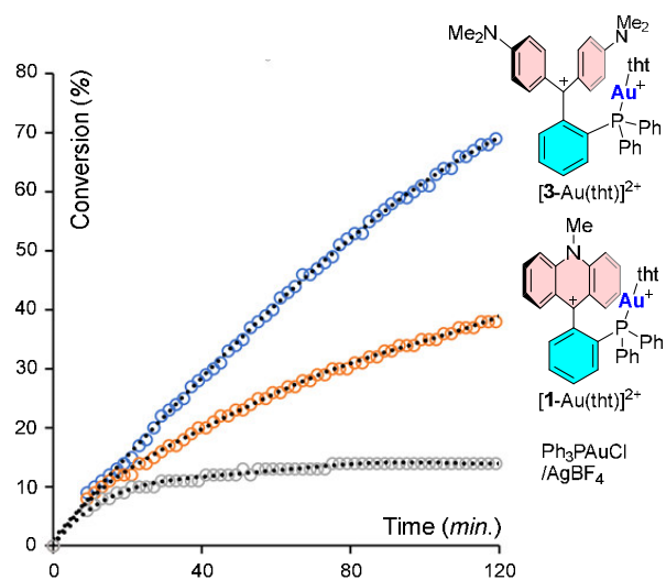
Fig 5. Conversion of propargyl amide 5 into 6 as a function of time with different catalysts.
