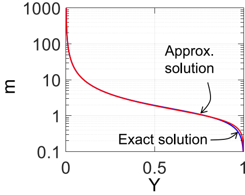
Fig. 4. Comparison of accuracy of Eq. (63) in approximating the exact solution, Eq. (62).
