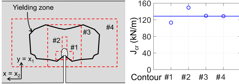
Fig. 6. J -integrals on different contours (the cross-hatched area indicates the fracture process zone, FPZ), computed on the specimens with D = 24 mm and transverse thickness b = 25 mm (Fig. 5d,e,f). Path 3 and 4 indicate path-independence, but 1 and 2 (which cross into the FPZ) do not.
