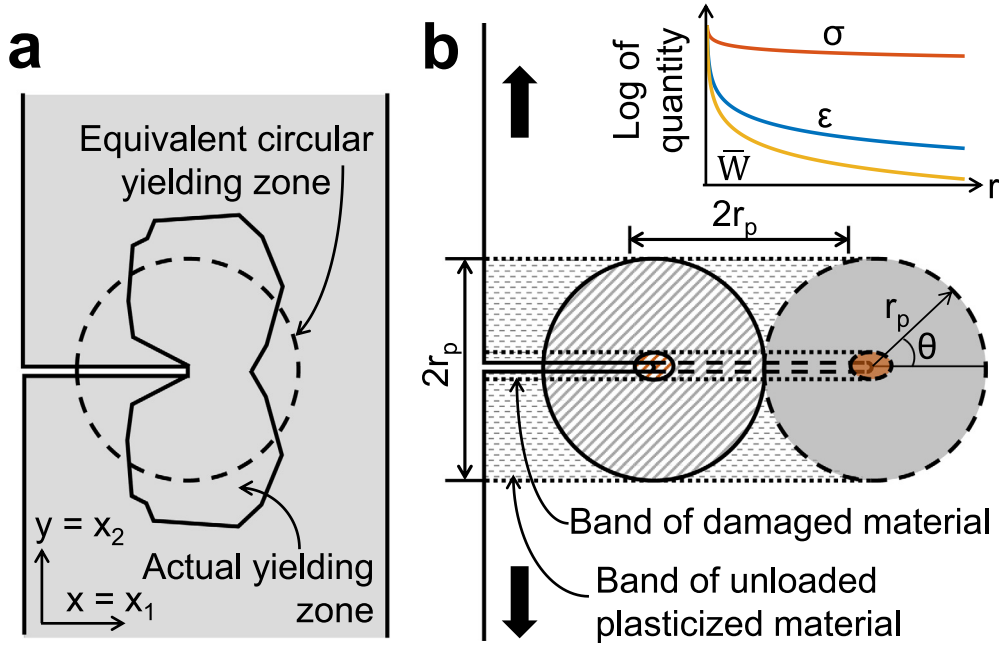
Fig. 3. (a) Actual and equivalent yielding zones with the same area (or volume), as indicated by FE analysis using von-Mises type plastic-hardening constitutive law; (b) Propagation of the equivalent yielding zone as crack grows.
