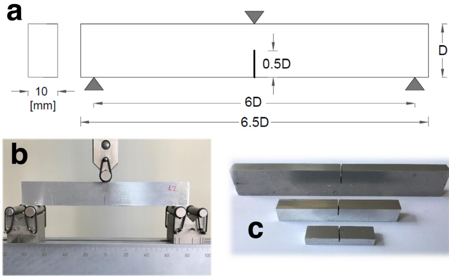
Fig. 8. (a) Schematic and (b) actual setup of notched three-point-bend tests; (c) Geometrically-scaled specimens with the same transverse thickness and various depths, D = 6, 12, 24 mm (specimens with D = 48 mm were tested but not shown here).
