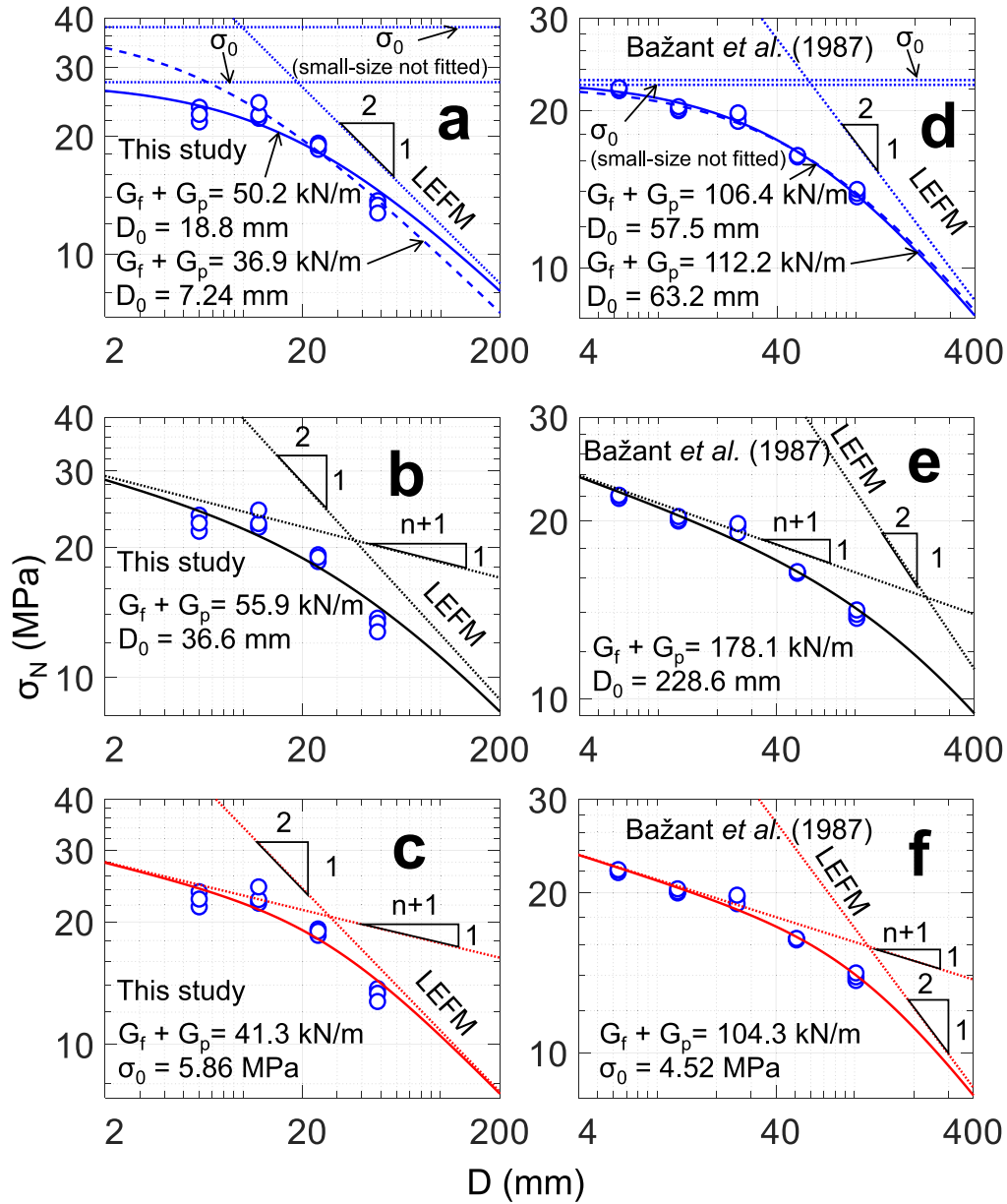
Fig. 5. Optimum fits of size effect law to test result on aluminum beams based on: (a,d) Eq. (53); (b,e) Eq. (57) (c,f). The transverse thickness of specimens was 10 mm (a,b,c), and 25.4 mm (1 in.) [30] (d,e,f).
