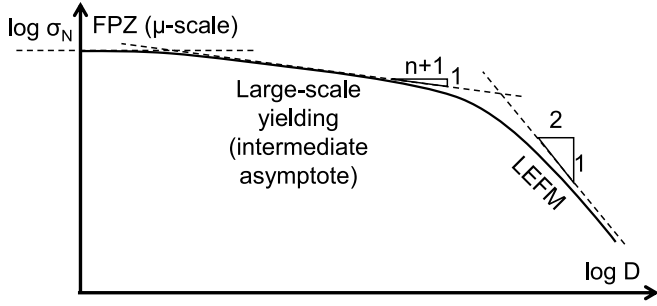
Fig. 7. Micron-scale asymptote for specimens with sizes comparable to process zone size (volume confined within slip planes or grain boundaries), and transition to intermediate asymptote and terminal asymptote.
