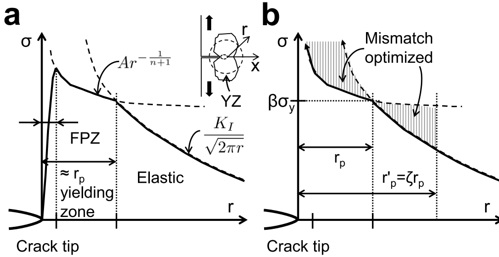
Fig. 2. Schematic radial stress profiles; (a) intersection of yielding and elastic zones; and (b) mismatch areas (cross-hatched) for equilibrium matching of both zones by virtual work.
