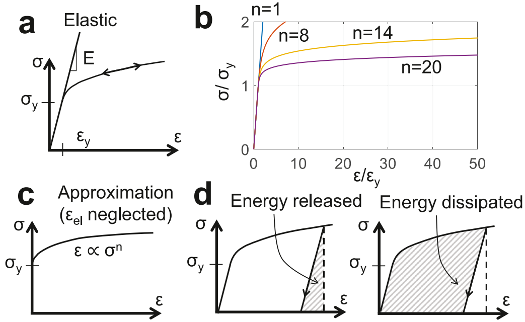
Fig. 1. (a) Stress-strain behavior of the deformation theory of plasticity (nonlinear elasticity); (b) Elasto-plastic constitutive law with different n ; (c) Approximation of total stress-strain relation by plastic stress-strain relation (elastic strain is neglected); and (d) Partition of strain energy at unloading into released and dissipated.
