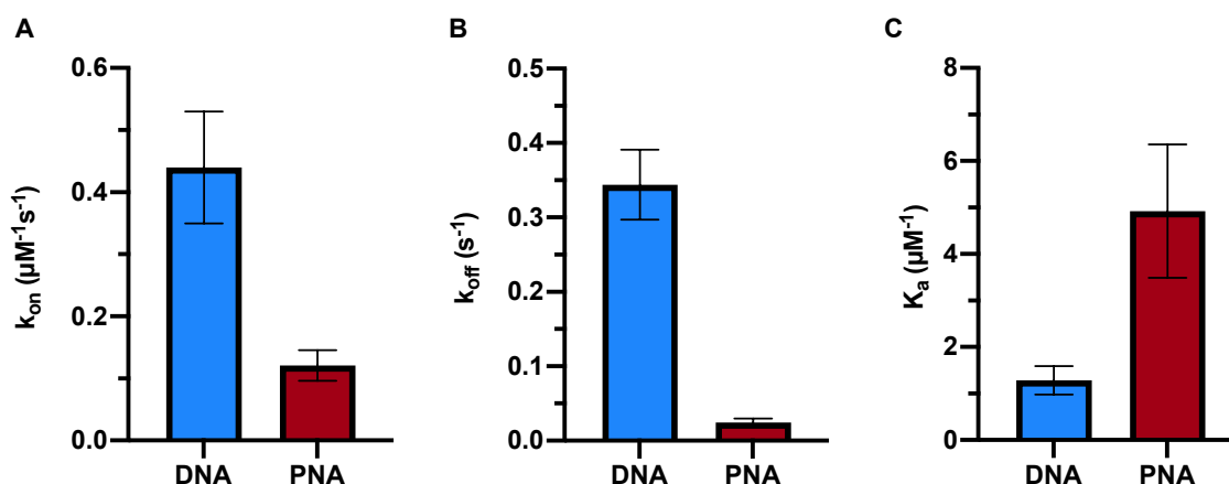
Figure 3: Comparison of 9-mer DNA and PNA target hybridization kinetics showing A) association rate constant, B) dissociation rate constant, and C) association constant. All data was measured at 450 mM NaCl at 22.5°C. PNA sequence: {}^C TGT ATC CAT ^N – TAMRA. DNA sequence: 3'-TGT ATC CAT-TAMRA-5'. Error bars represent 2 times the standard error of the mean (n=3). Error bars represent 2 times the standard error of the mean from 3 separate experimental trials, each probing 2500 \pm 700 immobilized probe molecules.
