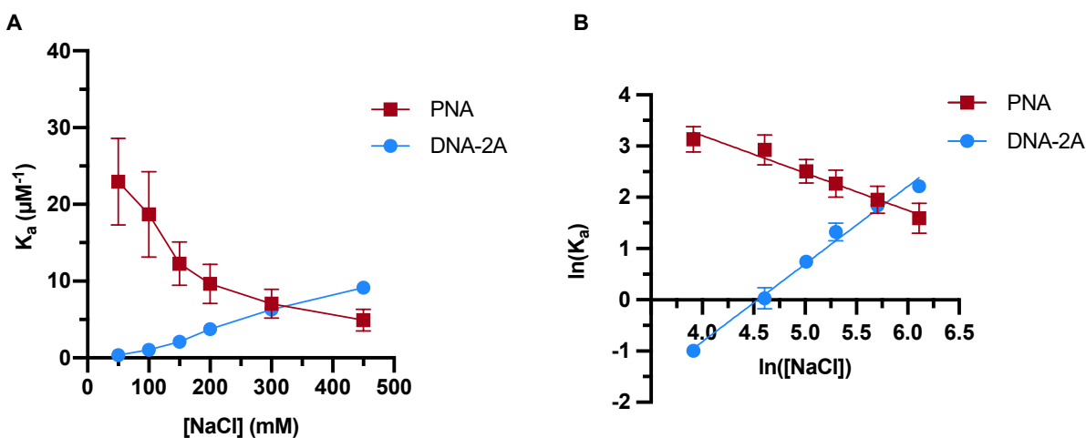
Figure 5: Trends in duplex association constant for PNA and DNA-2A with ionic strength at 22.5°C with A) linear plot and B) Leipply type analysis of log-log plot.
