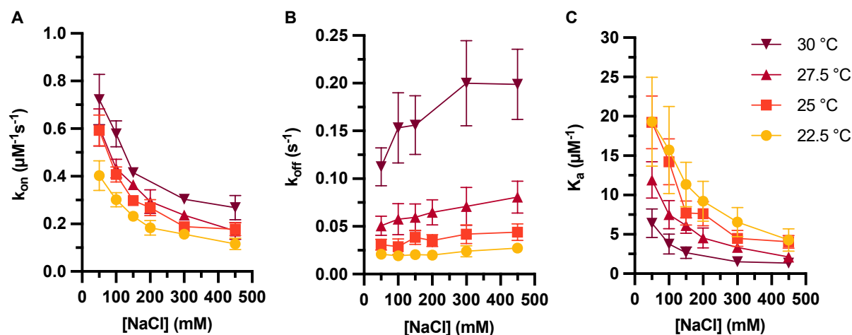
Figure 6: PNA target duplex formation kinetics and association constant at varying temperature and ionic strength, showing A) association rate constant, B) dissociation rate constant, and C) association constant. Rate constants determined on data sets with an average of 960 \pm 70 molecules each. Error bars represent two standard errors estimated as described in Supporting Information.
