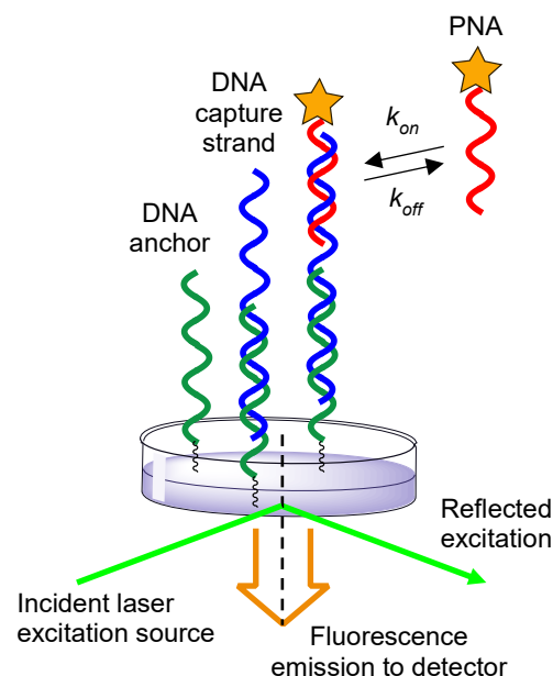
Figure 2: Schematic of experimental setup illustrating the anchor DNA, immobilized DNA capture strand, and diffusing PNA probe.
