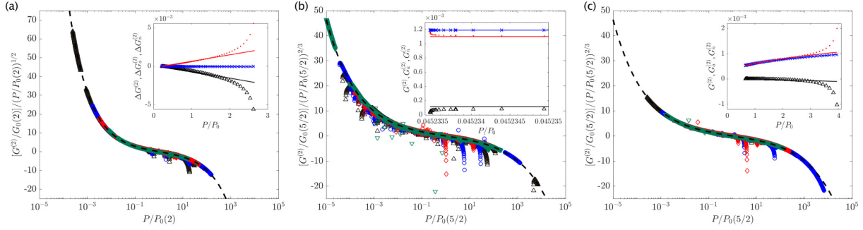
FIG. 9. (a) (G^{(2)}/G_0)(P/P_0)^{-1/2} vs P/P_0 for packings with \alpha = 2 in the second geometrical family following a point or jump change in the contact network. (G^{(2)}/G_0)(P/P_0)^{-2/3} is plotted vs P/P_0 for packings with \alpha = 5/2 in the second geometrical family following (b) a point change or (c) a jump change in the contact network. In (a)–(c), several system sizes are shown: N = 32 (black upper triangles), 64 (blue circles), 128 (red diamonds), 256 (green downward triangles), and 512 (magenta asterisks). The dashed lines in (a)–(c) give Eq. (4) for \alpha = 2 in (a) and 5/2 in (b) and (c). In the insets to (a)–(c), we show \Delta G^{(1)} = G^{(1)}(P/P_0) - G^{(1)}(0) or G^{(1)}(P/P_0) (black upward triangles), \Delta G_n^{(1)} = G_n^{(1)}(P/P_0) - G_n^{(1)}(0) or G_n^{(1)}(P/P_0) (red dots), and \Delta G_a^{(1)} = G_a^{(1)}(P/P_0) - G_a^{(1)}(0) or G_a^{(1)}(P/P_0) (blue \times ) with best fits to Eq. (2) (black, red, and blue solid lines, respectively) for an example N = 32 packing with \alpha = 2 [inset to (a)] and 5/2 [insets to (b) and (c)].
