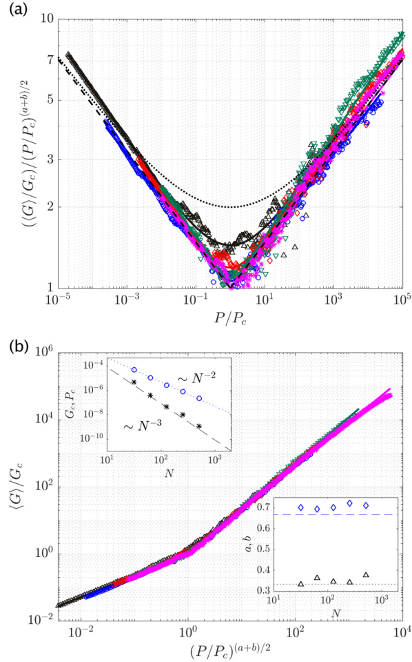
FIG. 13. (a) Ensemble-averaged shear modulus ((G)/G_c)(P/P_c)^{-(a+b)/2} vs P/P_c for jammed disk packings with \alpha = 5/2 and system sizes N = 32 (black upward triangles), 64 (blue circles), 128 (red diamonds), 256 (green downward triangles), and 512 (magenta asterisks). The dashed lines have slopes equal to -1/6 and 1/6 . The dotted line gives Eq. (6). (b) (G)/G_c plotted vs (P/P_c)^{(a+b)/2} for the same data in (a). The solid lines in (a) and (b) are fits to Eq. (7) with p = 2-15 for system sizes N = 32-512 . The upper left inset shows P_c (black asterisks) and G_c (blue circles) vs N . The dotted and dashed lines have slopes equal to -2 and -3 , respectively. The lower right inset gives the exponents, a (black upper triangles) and b (blue diamonds), used in fits to Eq. (7) vs N . The horizontal dotted and dashed lines indicate a = 1/3 and b = 2/3 , respectively.
