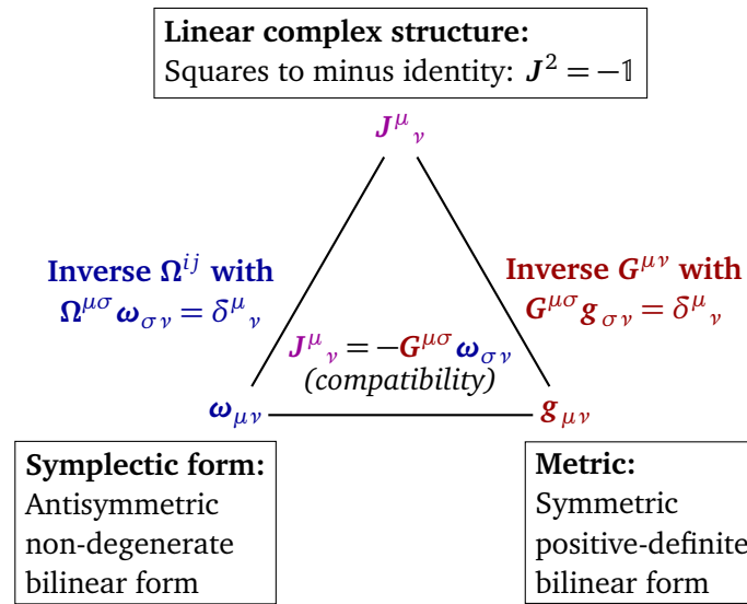
Figure 1: Triangle of Kähler structures . This sketch illustrates the triangle of Kähler structures, consisting of a symplectic form \omega , a positive definite metric g and a linear complex structure J . We also define the inverse symplectic form \Omega and the inverse metric G .
