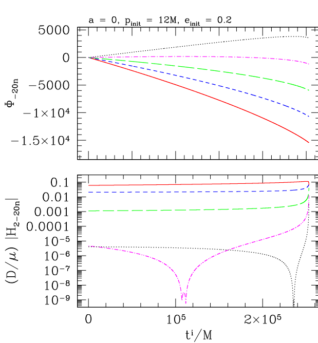
FIG. 9. Some voices with l = 2 and m = -2 which contribute to h_+ for the small-eccentricity case shown in Fig. 2. Colors and definitions are exactly as in Fig. 8. The behavior of modes with n = 3 and n = 4 are interesting: During the inspiral, there are moments at which the phase evolution reverses direction, corresponding to the voice’s instantaneous frequency changing sign. The amplitudes corresponding to these voices pass through zero at times very close to these moments. The zero passage of these amplitudes leads to the sharp appearance that we see here. The real and imaginary parts of H_{2-23} and H_{2-24} are perfectly smooth.
