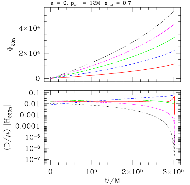
FIG. 10. Some voices with l = 2, m = 2 which contribute to the large-eccentricity waveform shown in Fig. 2. The top panel shows the voices’ phase; the lower panel shows their amplitudes. Solid (red) curves are data with n = 0 , short-dashed (blue) curves are n = 3 , long-dashed (green) curves are n = 6 , dot-dashed (magenta) curves are n = 9 , and dotted (black) curves are n = 12 . In contrast to the small-eccentricity case, the voice with n = 12 does not dominate over most of the inspiral. In fact, of the voices shown, the one which starts weakest ( n = 3 ) evolves to become the loudest by the end of inspiral. Nonetheless, all amplitudes and phases evolve in a smooth and simple way, just as in the low-eccentricity case.
