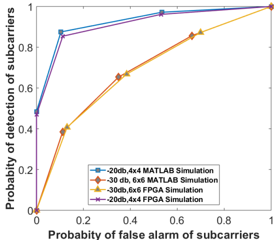
Figure 7: ROC curve of MATLAB simulations and FPGA Implementation platform.
