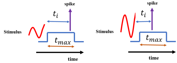
Figure 2: TTFS encoding.
