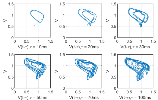
Figure 4: Phase Portrait.
