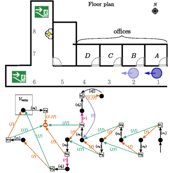
Fig. 4: A robot moves toward the charging station, while avoiding stairs. The figure below shows the p-graph of this planning problem.
