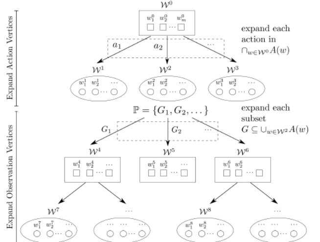
Fig. 3: The robot's belief tree. Action and observation vertices, visualized as boxes and circles respectively, have different expansions.
