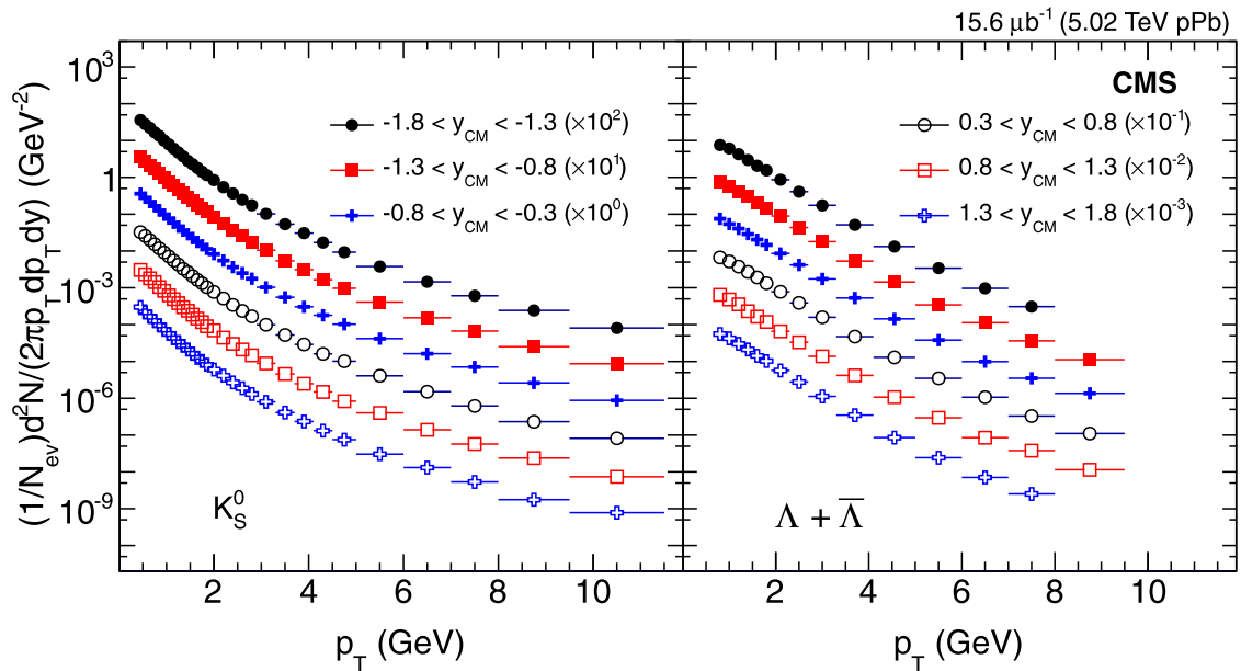
FIG. 5. The invariant p_T -differential spectra of K_S^0 (left) and \Lambda + \bar{\Lambda} (right) particles for -1.8 < y_{CM} < -1.3 , -1.3 < y_{CM} < -0.8 , -0.8 < y_{CM} < -0.3 , 0.3 < y_{CM} < 0.8 , 0.8 < y_{CM} < 1.3 , and 1.3 < y_{CM} < 1.8 in pPb collisions at \sqrt{s_{NN}} = 5.02 \text{ TeV} . Spectra in different y_{CM} ranges are scaled by factors of powers of 10, with -0.8 < y_{CM} < -0.3 not scaled. The vertical bars correspond to statistical uncertainties, which are usually smaller than the marker size, while the horizontal bars represent the bin width.
