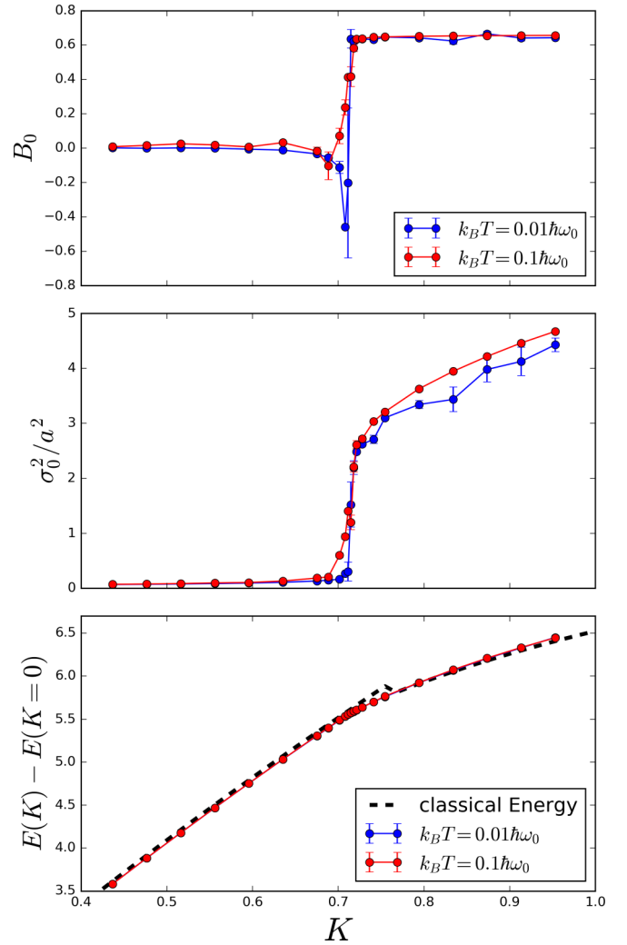
FIG. 10. Effect of temperature. Central particle Binder cumulant (top), variance (middle), and energy (bottom) for two different temperatures as specified in the legend.
