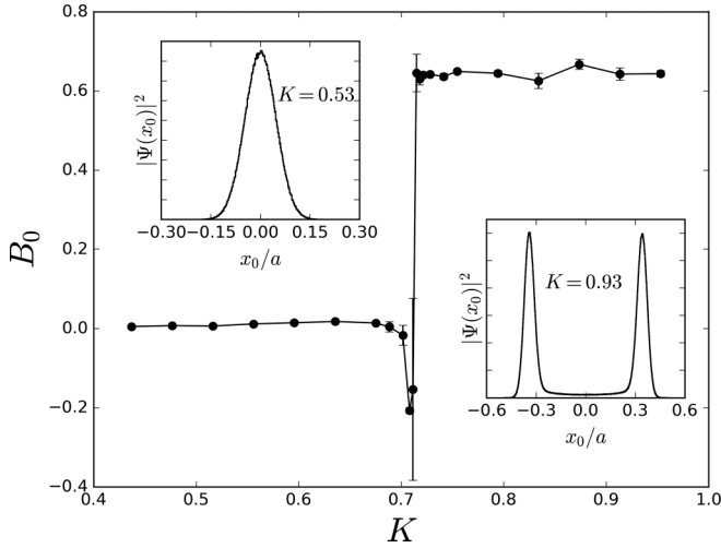
FIG. 2. Characterizing quantum effects via the Binder cumulant B_0 in a near-commensurate situation ( \Delta \approx 0.22 ). Behavior of B_0 [Eq. (5)] for the probability distribution of the central particle as a function of the scaled optical-lattice depth K in a fully commensurate system. Notice the sharp increase of B_0 at the value K \simeq K_c \simeq 0.7 . For low values of the potential, B_0 \simeq 0 , indicating a Gaussian-like distribution, while for large K values we find B_0 \simeq 2/3 , characteristic of a bimodal distribution. Upper left inset: Gaussian-like probability distribution (modulus squared of the single particle wave function) for K < K_c . Lower right inset: bimodal distribution for K > K_c .
