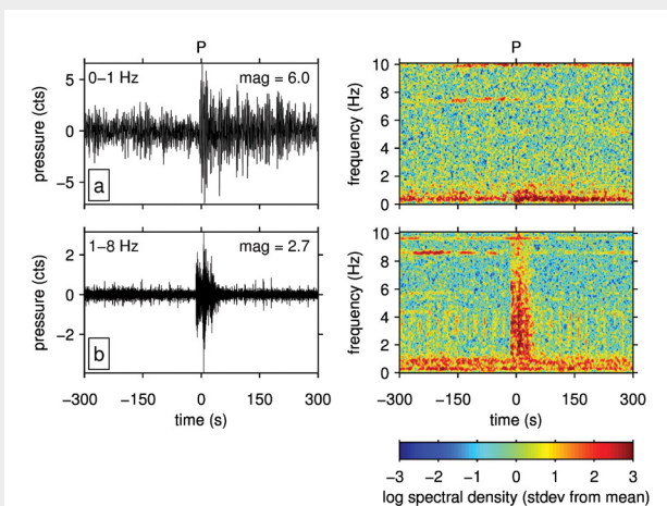
Figure 4. Seismic events detected at a 700 m depth offshore of San Diego, CA, during the recovered deployments of MERMAID-001. a: Only the large (magnitude [mag] 6) event is from a distant source 5,170 km from the epicenter as measured along the surface of the Earth and is thereby suited to map seismic wave speed variations in the Earth's mantle. b: a nearby (144 km epicentral distance) smaller (magnitude 2.7) crustal earthquake. Left column: filtered pressure records aligned on the first-arriving seismic "P" wave. Right column: Fourier spectrograms. These reveal how earthquake propagation over long distances filters out the high frequencies. Pressure conversions due to the close-by earthquake remain prominent in the range of 0-10 Hz, whereas the distant quake registers as a relatively small blip of power around 0.5 Hz. MERMAID's onboard processing unit recognizes these differences and is now tuned to preferentially report large earthquakes. The horizontal bands of energy are caused by nonseismic oceanic acoustic noise. Reproduced from Simons et al., 2009, with permission.
