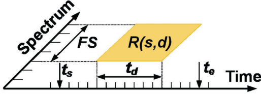
Fig. 5. A scheduled lightpath demand.
