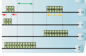
Fig. 2. A 19-core fiber with lightpaths established in the various cores.
