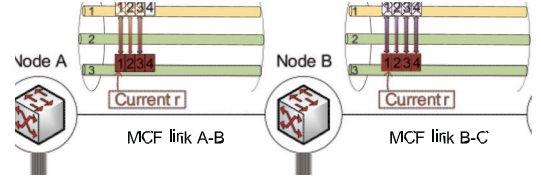
Fig. 10. Estimating inter-core crosstalk for new and existing lightpaths.
