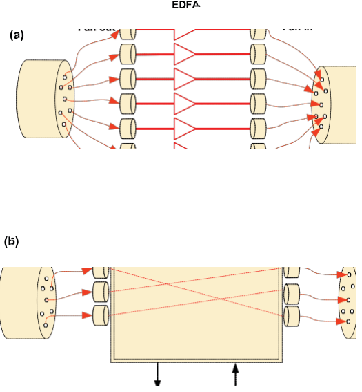
Fig. 4. Architecture of amplification and switching systems in the MCF-SDM network.
