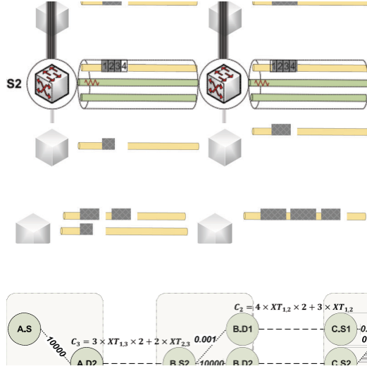
Fig. 9. Creating an auxiliary graph based on a combination of TW and SW.
