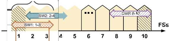
Fig. 6. Spectrum windows (SWs) in a fiber link.
