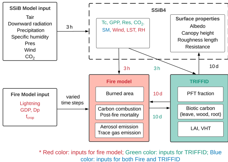
Figure 1. Schematic diagram of fire model coupling in SSiB4/TRIFFID-Fire (Tair: air temperature; Pres: surface pressure; Dp: population density; f_{\text{crop}} : crop fraction; Tc: canopy temperature; Res: autotrophic respiration; SM: soil moisture; LST: land surface temperature; RH: relative humidity; VHT: vegetation height)
