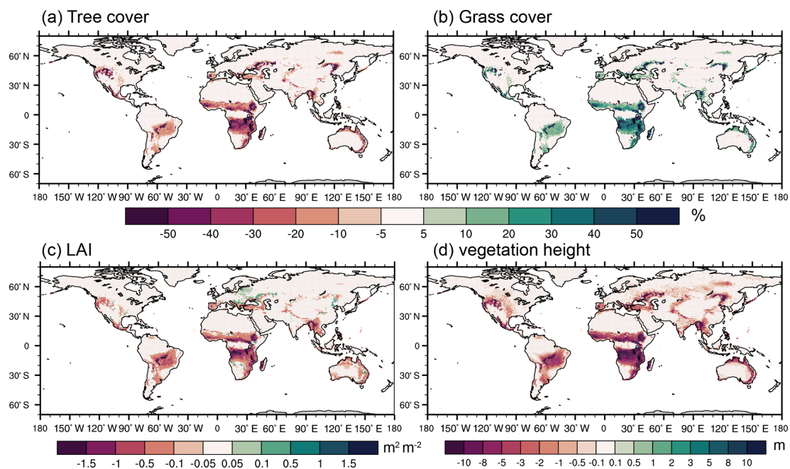
Figure 11. Differences in (a) tree cover (BET, NET, and BDT; %), (b) grass cover ( \text{C}_3 and \text{C}_4 ; %), (c) LAI ( \text{m}^2 \text{m}^{-2} ), and (d) vegetation height (m) in SSiB4/TRIFFID-Fire averaged over 2000–2014 between FIRE-ON and FIRE-OFF.
