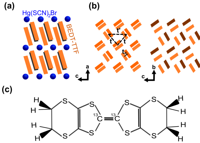
FIG. 1. (a) Structure of \kappa -HgBr, which consists of alternating layers of anions (blue) and (BEDT-TTF) 2 cations (orange) along the a axis. (b) Intralayer arrangement of cations in the bc plane with the respective transfer integrals, as indicated. While the left side depicts a strongly dimerized structure ( t_d \gg t, t' ), giving rise to Mott-insulating behavior, weakly bound dimers (right) pronounce intersite Coulomb interaction, with a tendency to charge order. Charge-rich and -poor molecules are distinguished by light and dark colors, respectively. (c) The two central carbon atoms of BEDT-TTF have been spin labeled by ^{13}\text{C} for NMR investigations.
