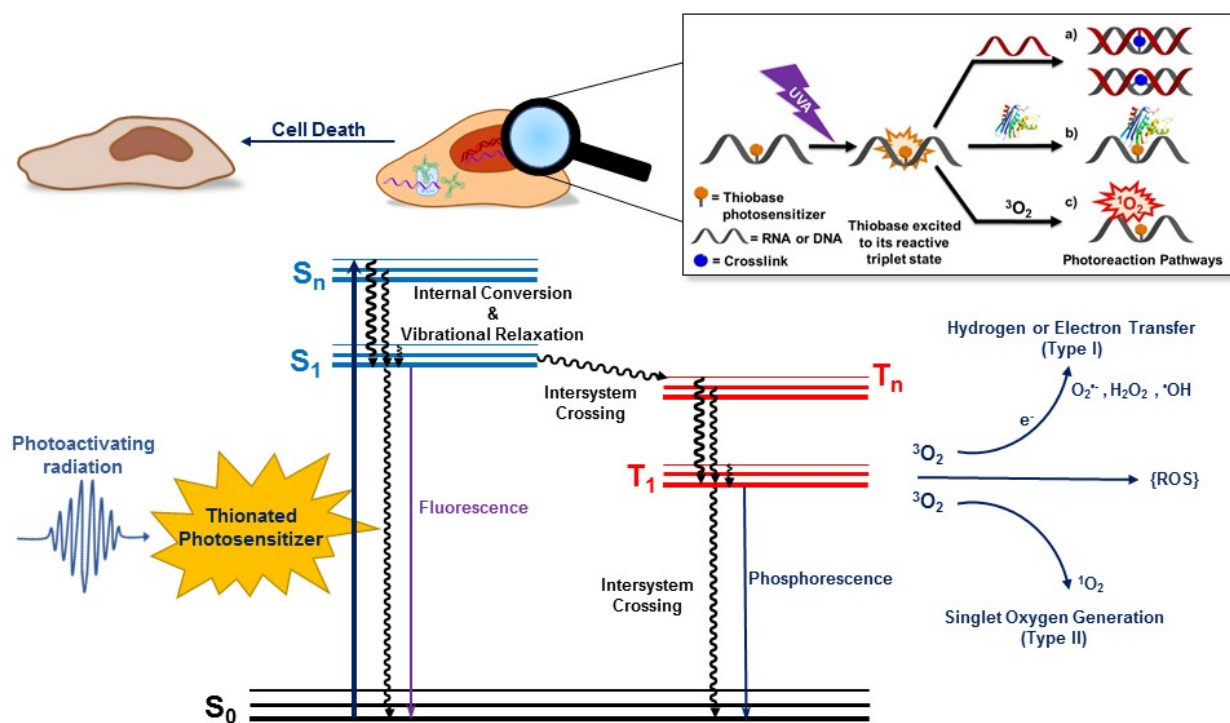
Figure 1. (Top) Generic UVA-induced reaction mechanisms of the thioether derivatives, which includes photocrosslinking reactions with (a) DNA or (b) proteins, and (c) triplet-energy transfer to generate molecular oxygen in its excited singlet state. Electron transfer from the triplet state of the thioether to molecular oxygen to generate the superoxide anions and other ROS such as hydrogen peroxide and hydroxyl radicals is also possible, but not shown. These reactions can lead to cell death. (Bottom) Jablonski electronic-energy diagram depicting the primary events leading to Type I and Type II photosensitized reactions, which eventually can result in oxidatively-induced cell damage. S_0 represents the ground electronic state of the photosensitizer, S_n and T_n represent upper excited singlet and triplet states, respectively, and S_1 and T_1 are the lowest-energy singlet and triplet states.
