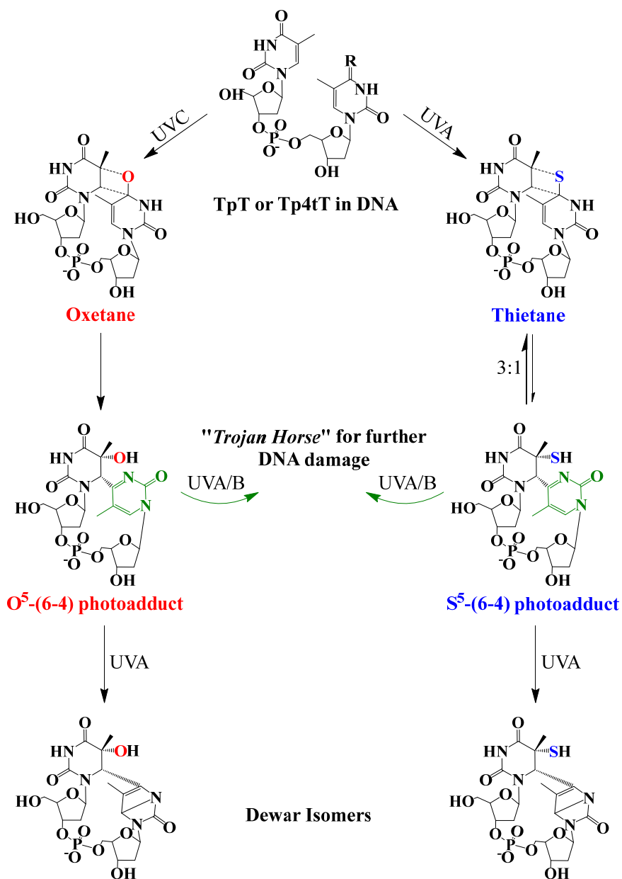
Figure 4. Photochemistry of adjacent thymine-thymine (TpT) or thymine-4-thiothymine (Tp4tT) in DNA upon UV irradiation (modified from refs. 43, 63, 66 ). Irradiation of TpT with UVC, or Tp4tT with UVA radiation, generates an oxetane or a thietane intermediate, respectively. The oxetane is highly unstable and spontaneously converts into the O 5 -(6-4) photoadduct (its ring-open form), whereas the thietane is more stable and exists as a 3:1 equilibrium between the thietane and its ring-open form; the S 5 -(6-4) photoadduct analog. Irradiation of the ring-open forms of both O 5 -(6-4) photoadduct and S 5 -(6-4) photoadduct with UVA/B radiation can convert them into their respective Dewar isomers or can excite the pyrimidone moiety (highlight with green color) to generate further damage to DNA. Note that metabolism of 4tThd into DNA can be thought as a “Trojan horse” to photoactivate cellular damage (see, Figure 1), while the formation of the S 5 -(6-4) photoadduct in cellular DNA can further generate DNA damage upon UVA/B excitation of
