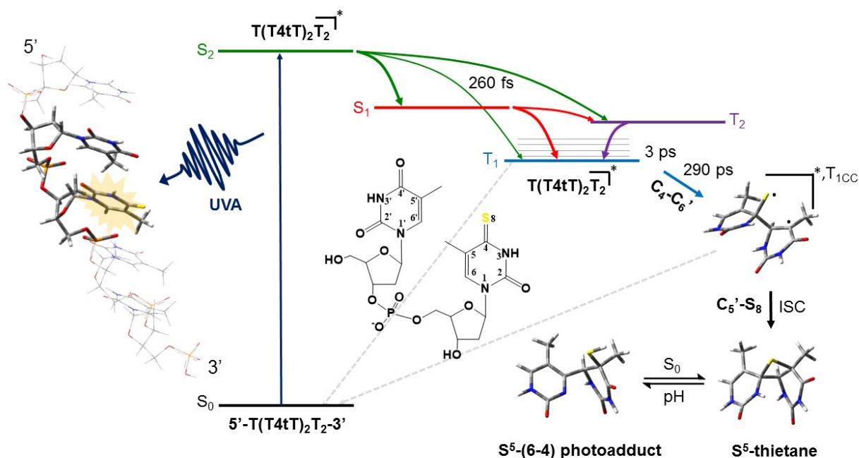
Figure 3. Proposed mechanism for the formation of the DNA (6-4) photoadduct in PBS at pH 7.4. A 4-thiothymine (4tT) base is highlighted with light orange in the single-stranded DNA sequence depicted to the left to imply that 4tT bases are selectively photoactivated by the UVA radiation. 4tThd and the thymidine 5' relative to the 4tT are represented as tube in the single-stranded DNA sequence, while the other nucleobases are depicted as wireframe in order to highlight the importance of having a thymine 5' relative to the 4tT for the reaction to occur. Figure reproduced from ref. 63 .
