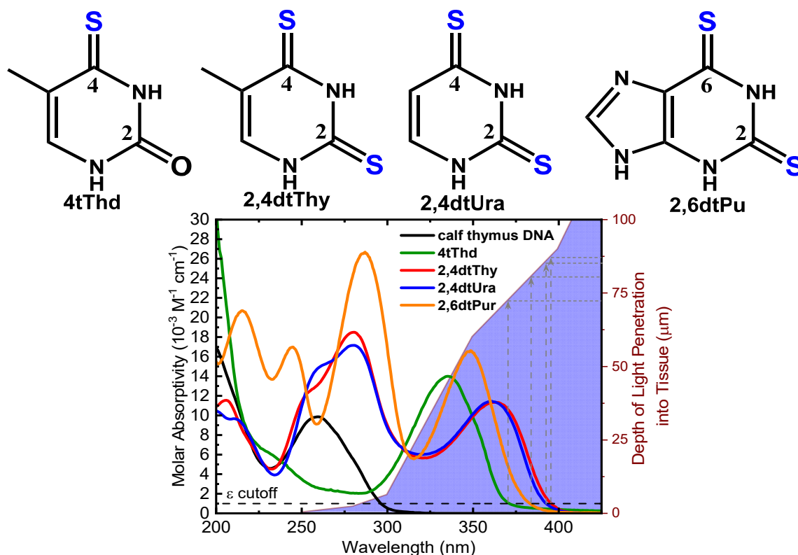
Figure 2. Molecular structure of the thiobases and the molar absorptivity spectra of calf thymus DNA, 4tThd, 2,4dtThy, 2,4dtUra and 2,6dtPu in PBS at pH 7.4 overlaid with depth of light penetration into fair Caucasian skin. 51-53
