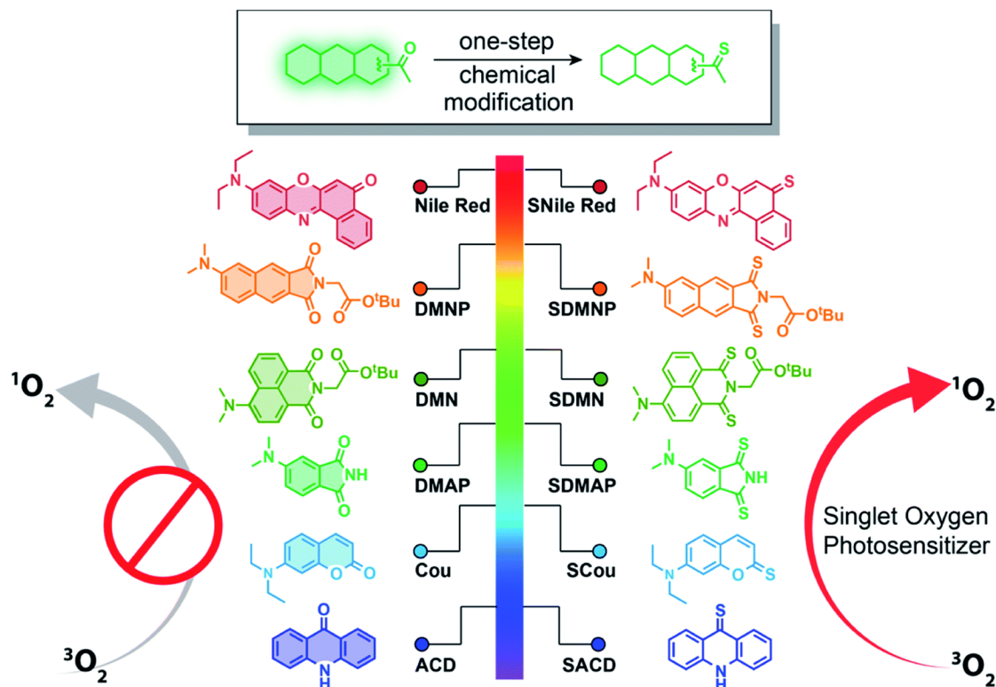
Figure 5. Thionation of a variety of biocompatible organic compounds can dramatically enhance their abilities to generate ROS. Illustrated are structures of the starting organic compounds (left) and thionated photosensitizers (right). Reproduced from ref. 80 .
