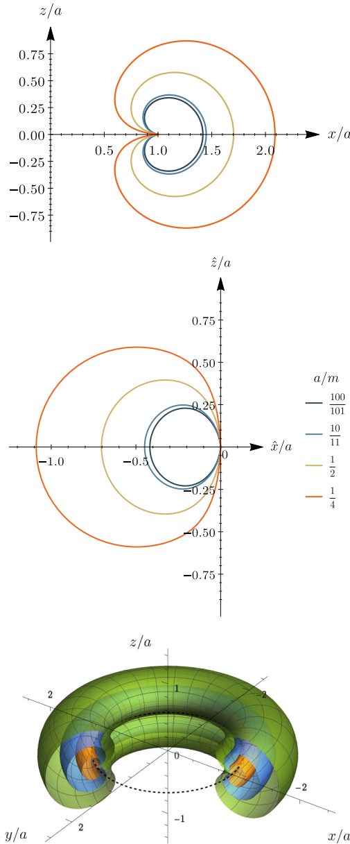
FIG. 3. Intersection of the boundary of the causality-violating region (i.e., the region with closed timelike-or-lightlike curves) with the half-plane \{x > 0, t = 0, y = 0\} in Kerr-Schild coordinates (top) and the coordinates (3.16) (middle), and the three-dimensional boundary close to the singular ring in Kerr-Schild coordinates (bottom), all in the negative- \tilde{r} region for different values of a/m ( a/m = 1/2 corresponds to green, 1 to blue, and 2 to orange/yellow). The Killing vector \partial_\phi is timelike in the region bounded by the curve and null on the boundary. The ring is located at (1,0) on the top panel, at the origin in the middle panel, and on the dotted line in the bottom panel. Observe that the cusp in the top panel disappears in the middle panel.
