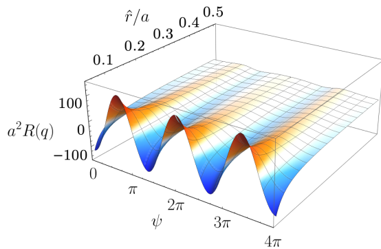
FIG. 6. Representative graph of the Ricci scalar a^2 R(q) as a function of \hat{r}/a \in [1/20, 1/2] and \psi \in [0, 4\pi] ; here a/m = 1/2 .
