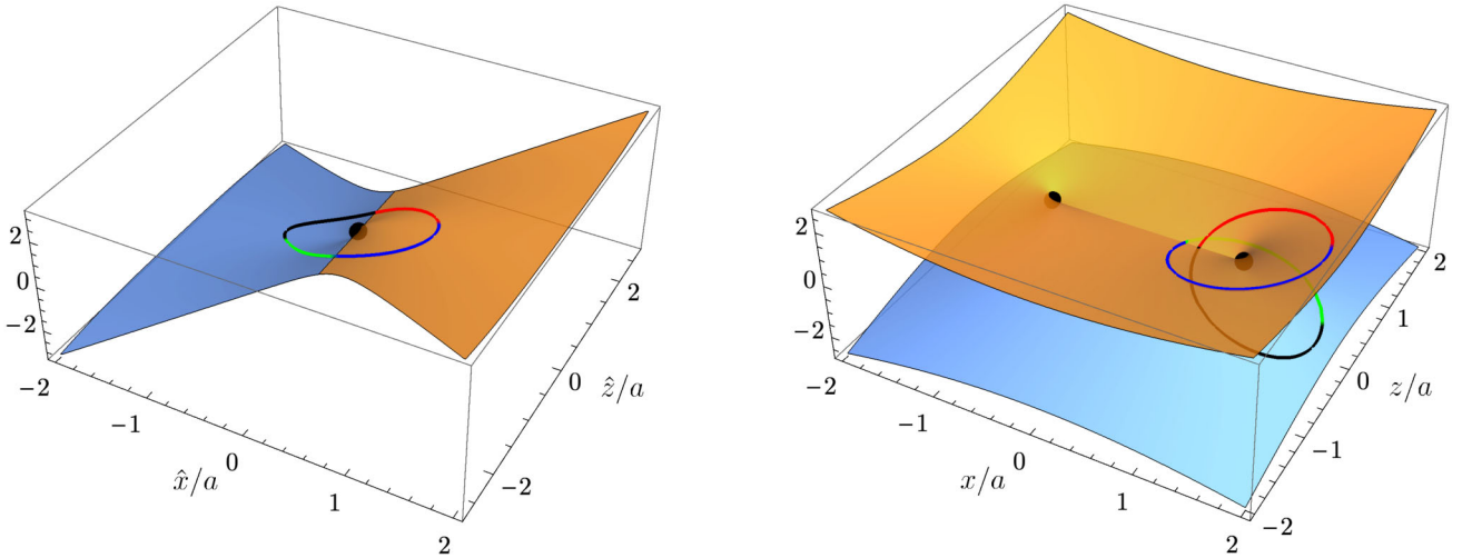
FIG. 2. Left: Graph of \tilde{r}/a over the image of the region \{x > 0, y = 0\} in (\hat{x}, \hat{z}) coordinates. Right: Graphs of \pm\tilde{r} , parametrized by (x, z) coordinates, over the hyperplane \{t = 0, y = 0\} . The location of the ring is indicated by black dots. The red curve corresponds to \psi \in [0, \pi) ( \tilde{r} > 0 ), the black curve to \psi \in (\pi, 2\pi] ( \tilde{r} < 0 ), the green curve to \psi \in (2\pi, 3\pi) ( \tilde{r} < 0 ), and the blue curve to \psi \in (3\pi, 4\pi] ( \tilde{r} > 0 ). Observe that the closed curve around the ring in the (\hat{x}, \hat{z}) coordinates on the left panel lifts to the curve shown on the right panel. The right plot incorrectly suggests that there is only one equatorial disk: a faithful visualization is provided by the left figure, which shows clearly that the extension contains two copies of the equatorial disk, which correspond to the sets \{\hat{x} = 0, \hat{z} > 0\} and \{\hat{x} = 0, \hat{z} < 0\} , as well as two copies of the exterior equatorial hyperplane, which correspond to the sets \{\hat{z} = 0, \hat{x} > 0\} and \{\hat{z} = 0, \hat{x} < 0\} .
