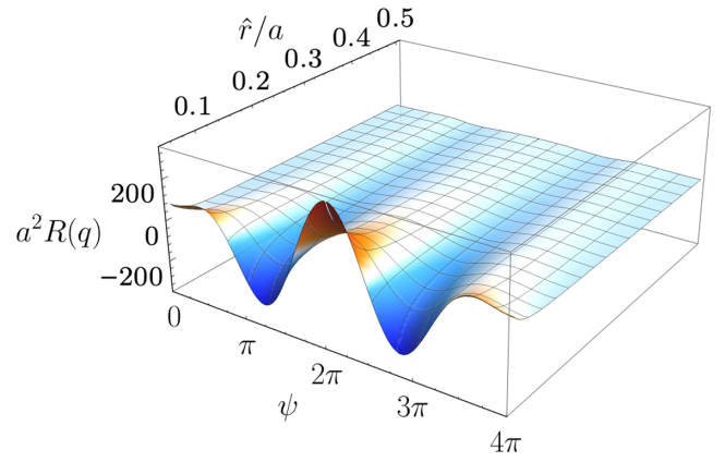
FIG. 8. The asymptotic form of the Ricci scalar of the quotient space metric q close to the singular ring changes for e \neq 0 ; see Eq. (7.30). Here we plot a representative graph of the Ricci scalar a^2 R(q) as a function of \hat{r}/a \in [1/20, 1/2] and \psi \in [0, 4\pi] , with a/m = 1/2 and e/m = 1 . Compare Fig. 6.
