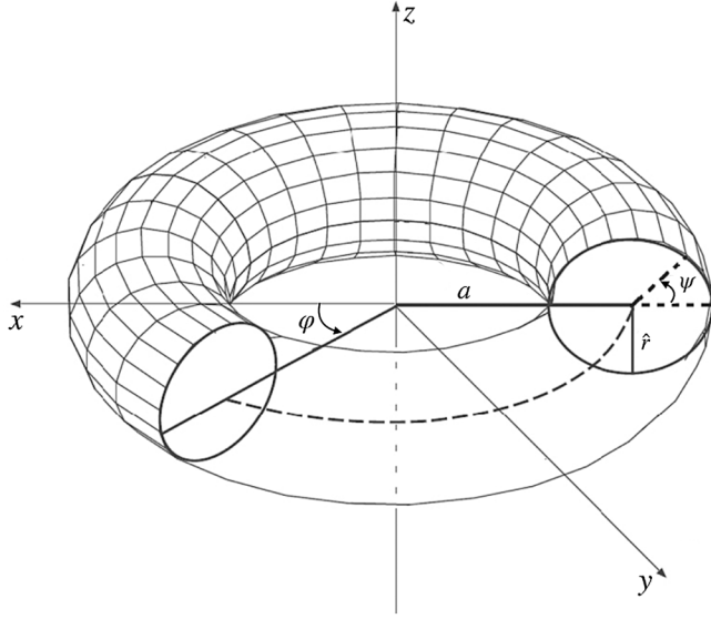
FIG. 1. Toroidal coordinates. The \hat{r} coordinate represents the minor radius of the torus, while the major radius is fixed at a . The angles \varphi and \psi are periodic, with \varphi adapted to rotations about the z axis, and \psi adapted to rotations about the curve that runs the circumference of the ring, shown by the dashed line. Clearly, for these coordinates to make sense, we must restrict \hat{r} < a .
