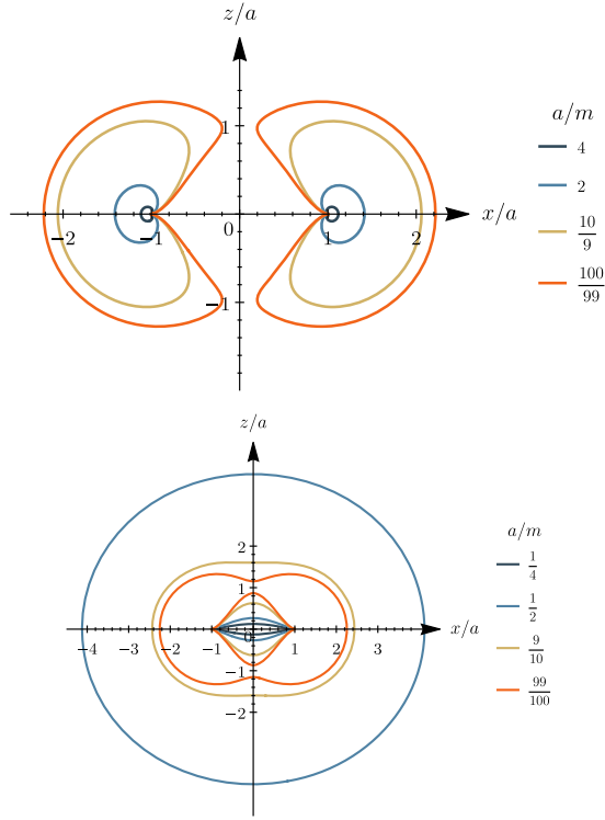
FIG. 4. The intersection of the boundary of the ergoregion (i.e., the region where the Killing vector \partial_{\tilde{t}} changes causal type) with the hyperplane y = 0 , in Kerr-Schild coordinates in the positive- \tilde{r} region, for a/m \in \{4, 2, 10/9, 100/99\} (top) and a/m \in \{1/4, 1/2, 9/10, 99/100\} (bottom). The Killing vector \partial_{\tilde{t}} is spacelike in the region bounded by the curves. We see that, near the ring, the boundary of the region where \partial_{\tilde{t}} is spacelike is connected for a \geq m (not embedded when a = m ), while it has two components for a < m .
