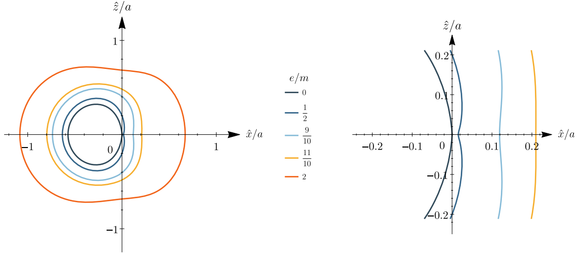
FIG. 7. In the hatted coordinates of Eq. (3.16), the Killing vector \partial_\phi is timelike in the region bounded by the curves of the left panel, with a zoom to the location of the ring (which sits at the origin of the coordinates) in the right panel. Here a = 2m/3 and e/m \in \{0, 1/2, 9/10, 11/10, 2\} .
