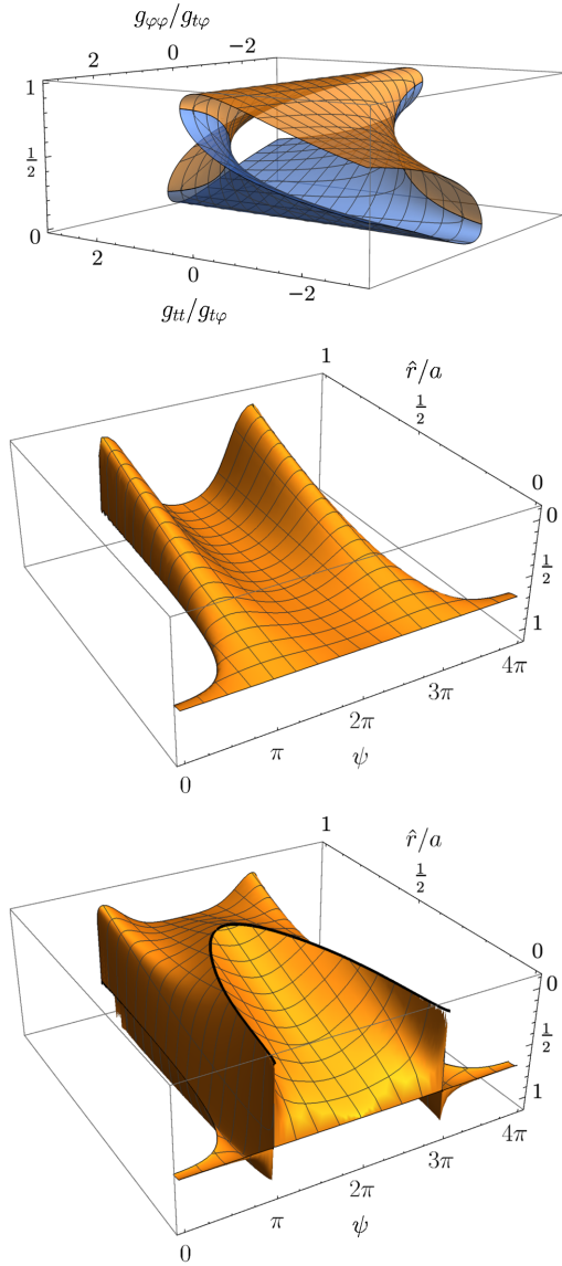
FIG. 5. The functions \cos^2(\alpha_+) \geq \cos^2(\alpha_-) as functions of g_{tt}/g_{t\varphi} and g_{\varphi\varphi}/g_{t\varphi} plotted over the region g_{tt}g_{\varphi\varphi} - g_{t\varphi}^2 < 0 and g_{t\varphi} \neq 0 (top) as well as the functions \cos(\alpha_+) (middle) and \cos(\alpha_-) (bottom), with the ordinate axis increasing downwards, as functions of \hat{r}/a and \psi with a/m = 1/2 . The set \cos(\alpha_-) = 0 coincides with the hypersurface \{g_{\varphi\varphi} = 0\} , on which the rotational Killing vector \partial_{\hat{\varphi}} = \partial_{\varphi} becomes null. The metric on the space of the orbits becomes spacelike beyond the curves at which the plots disappear.
