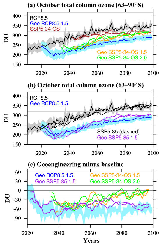
Figure 11. October averaged total column ozone between 63 and 90° S for different model experiments and ensemble members (different colors) (a, b). Grey and light blue areas show the standard deviation of the GLENS ensemble and the light grey line indicates 1980 values. (c) Differences between geoengineering and corresponding baseline experiments; the two black lines around zero indicate the standard deviation from the GLENS baseline simulations. A running mean over 5 years has been applied to the results.
