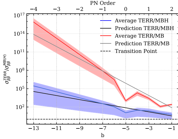
FIG. 8. Scaling relations discussed in Sec. VIA 1. The ratio \sigma_{\beta\beta}^{\text{TERR}}/\sigma_{\beta\beta}^{\text{MBH}} , calculated from the full Fisher simulations including the realistic noise curves shown in Fig. 2 and the IMRphenomPv2 waveform, is shown in blue. The empirically measured trend is derived from averaging the constraints from each terrestrial network and each population model, then calculating the ratios of every combination of terrestrial network and SOBH model against each MBH heavy-seeding model. The blue line shows the mean ratio, and the blue shaded region is the area bounded by the maximum and minimum ratios. The red line and the red shaded region refer instead to the ratio between the terrestrial-only constraints and the multiband constraints, i.e., \sigma_{\beta\beta}^{\text{TERR}}/\sigma_{\beta\beta}^{\text{MB}} . For this class of sources, we calculate the ratio for each population model and detector network, one at a time. That is, the terrestrial-only constraints from the S1 network derived from the SPOPS 265 model are compared against the multiband constraints from the S1 network and the SPOPS 265 model. The trends predicted analytically in the text are shown in black and grey for MBH and multiband sources, respectively. The trend lines we show for our predictions have been shifted along the y-axis to better compare the with the data.
