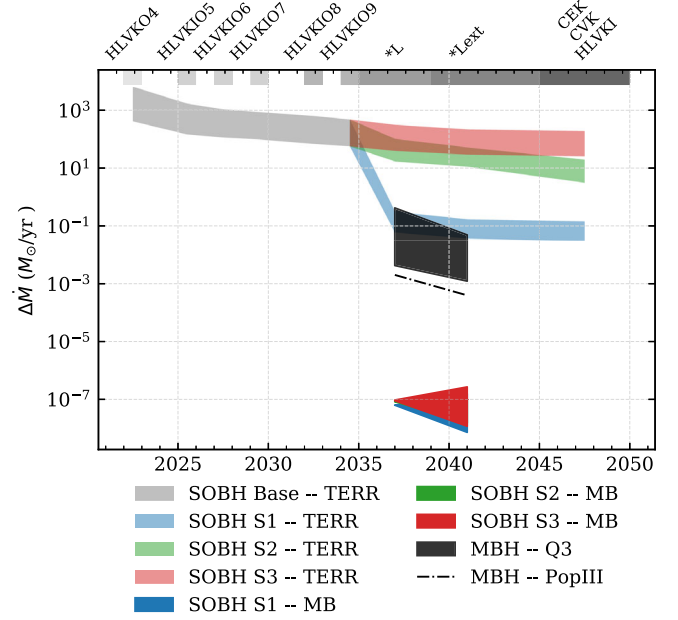
FIG. 22. Projected cumulative constraints on the rate of black hole evaporation \dot{M} , for the detector networks and population models examined in this paper. Our models predict multiband sources to perform the best from the three classes of sources examined in this paper, followed next by MBH observations by LISA. Terrestrial-only observations from the most optimistic scenario are competitive with LISA's MBH sources, but the other two scenarios considered in this work trail behind by 2–3 orders of magnitude.
