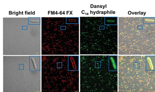
Fig. 3 Co-localization of FM4-64FX (5 μg mL -1 ) and dansyl C 14 hydrophile in tet R E. coli . Top panel: FM4-64FX was fixed after 5 minutes and dansyl C 14 hydrophile was fixed after 30 seconds. Bottom panel: FM4-64FX was fixed after 5 minutes and dansyl C 14 hydrophile was fixed after 5 minutes. The scale bars are 10 μm (approximately the width of the smaller boxes).
