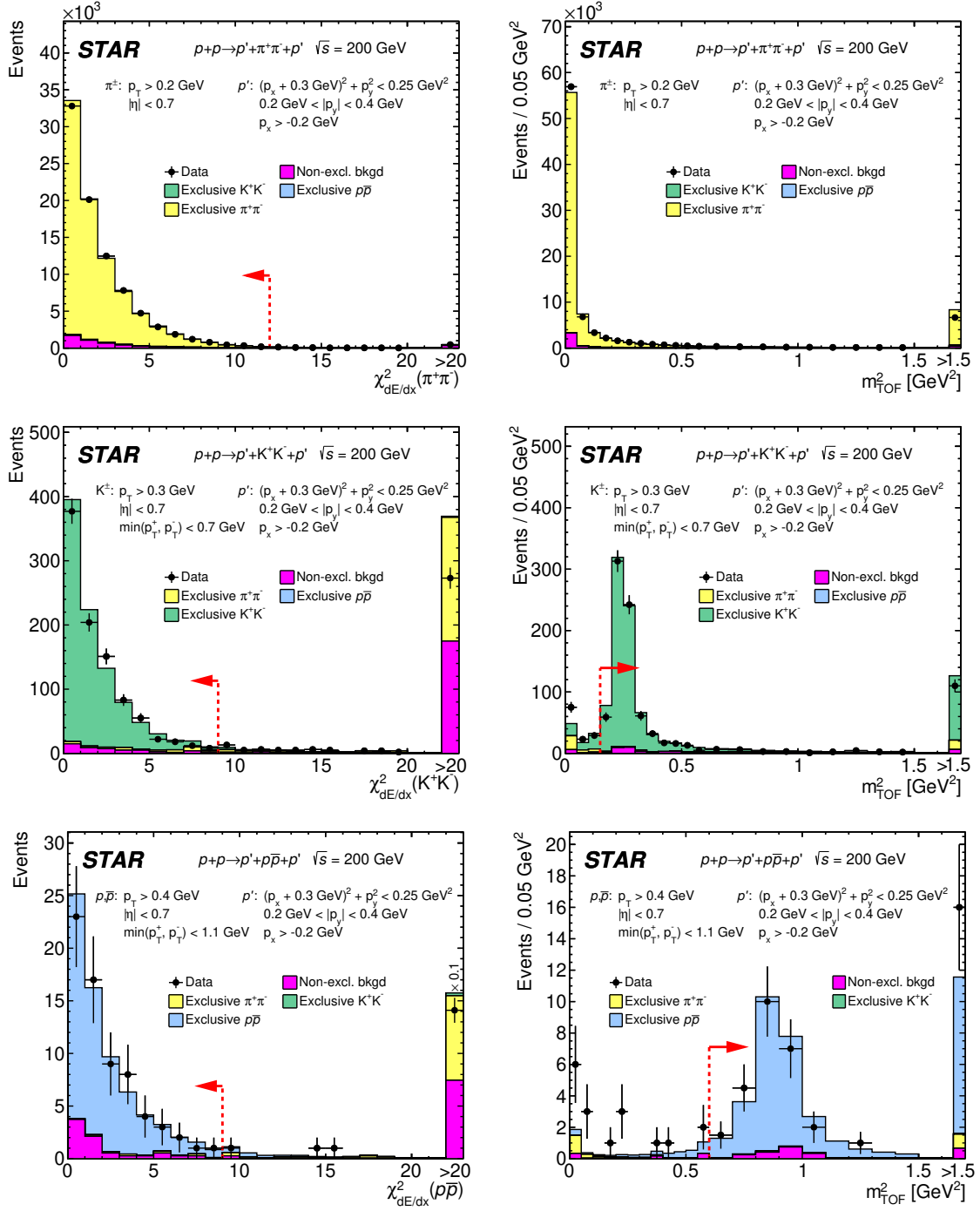
Figure 4. Distributions of \chi^2_{dE/dx} (left column) and m^2_{\text{TOF}} (right column) for exclusive \pi^+\pi^- (top), K^+K^- (middle) and p\bar{p} (bottom) candidates after final event selection. The dashed red line and arrow indicate the value of the cut imposed on the plotted quantity to select exclusive pairs of a given particle species. Yellow, blue and green histograms correspond to the fast exclusive MC simulation while magenta shows the estimated amount of non-exclusive background in the data.
