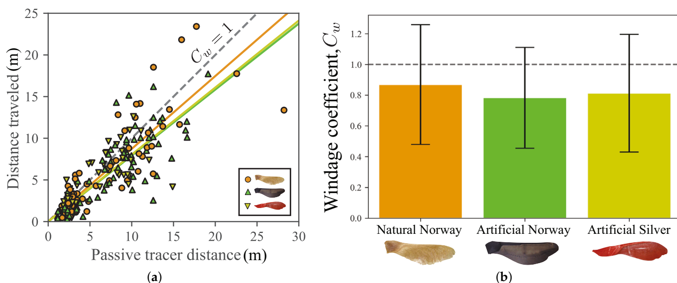
Figure 6. (a) The downwind distance traveled plotted against the effective downwind distance of a passive tracer during the same drop time. The ratio of these distances gives the windage coefficient, plotted in (b) for each of the three cases, with error bars giving standard deviation. The mean windage coefficient for each data set is shown by the straight line fit in (a).
